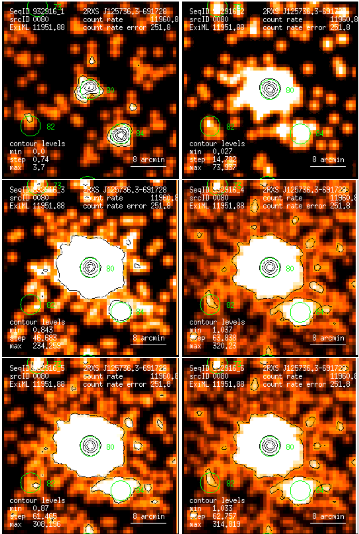
Figure 80: RASS 932916: detection 0080: band rate images, Gaussian filter: (1) PSPC channels 11 – 41, (2) 52 – 90, (3) 91 – 201, (4) 11 – 235, (5) 52 – 201, (6) 11 – 201. Broad band rates in counts/ks. Band rate contour levels in counts/ks/arcmin 2 .
