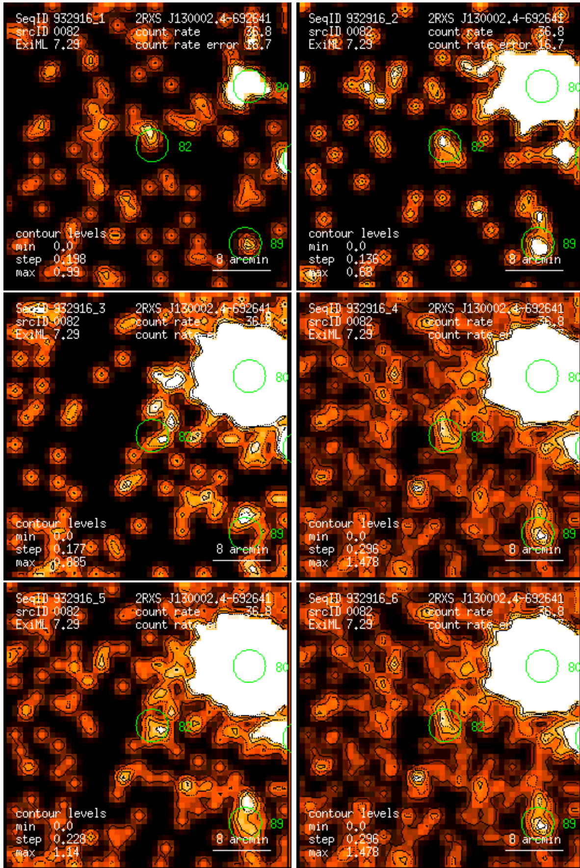
Figure 82: RASS 932916: detection 0082: band rate images, Gaussian filter: (1) PSPC channels 11 – 41, (2) 52 – 90, (3) 91 – 201, (4) 11 – 235, (5) 52 – 201, (6) 11 – 201. Broad band rates in counts/ks. Band rate contour levels in counts/ks/arcmin 2 .
