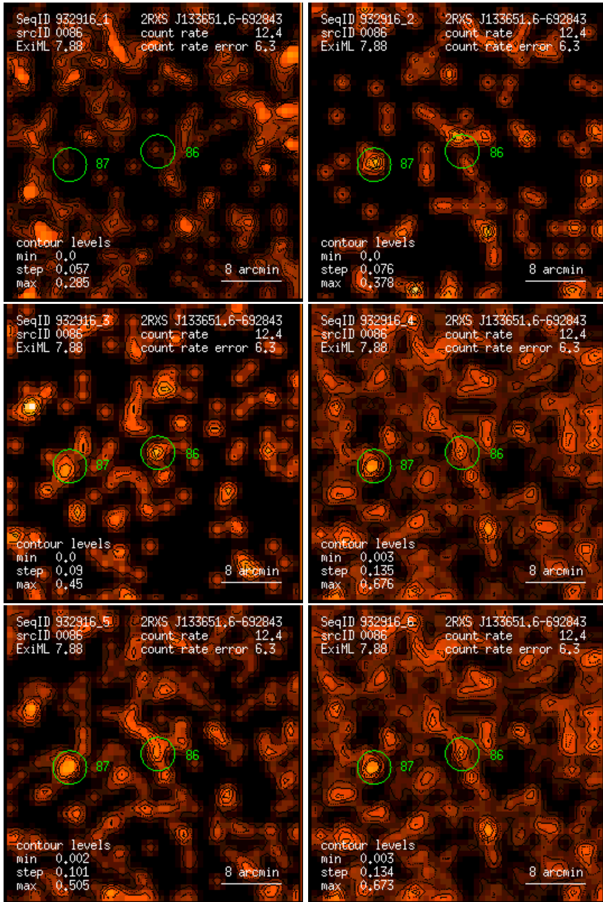
Figure 86: RASS 932916: detection 0086: band rate images, Gaussian filter: (1) PSPC channels 11 – 41, (2) 52 – 90, (3) 91 – 201, (4) 11 – 235, (5) 52 – 201, (6) 11 – 201. Broad band rates in counts/ks. Band rate contour levels in counts/ks/arcmin 2 .
