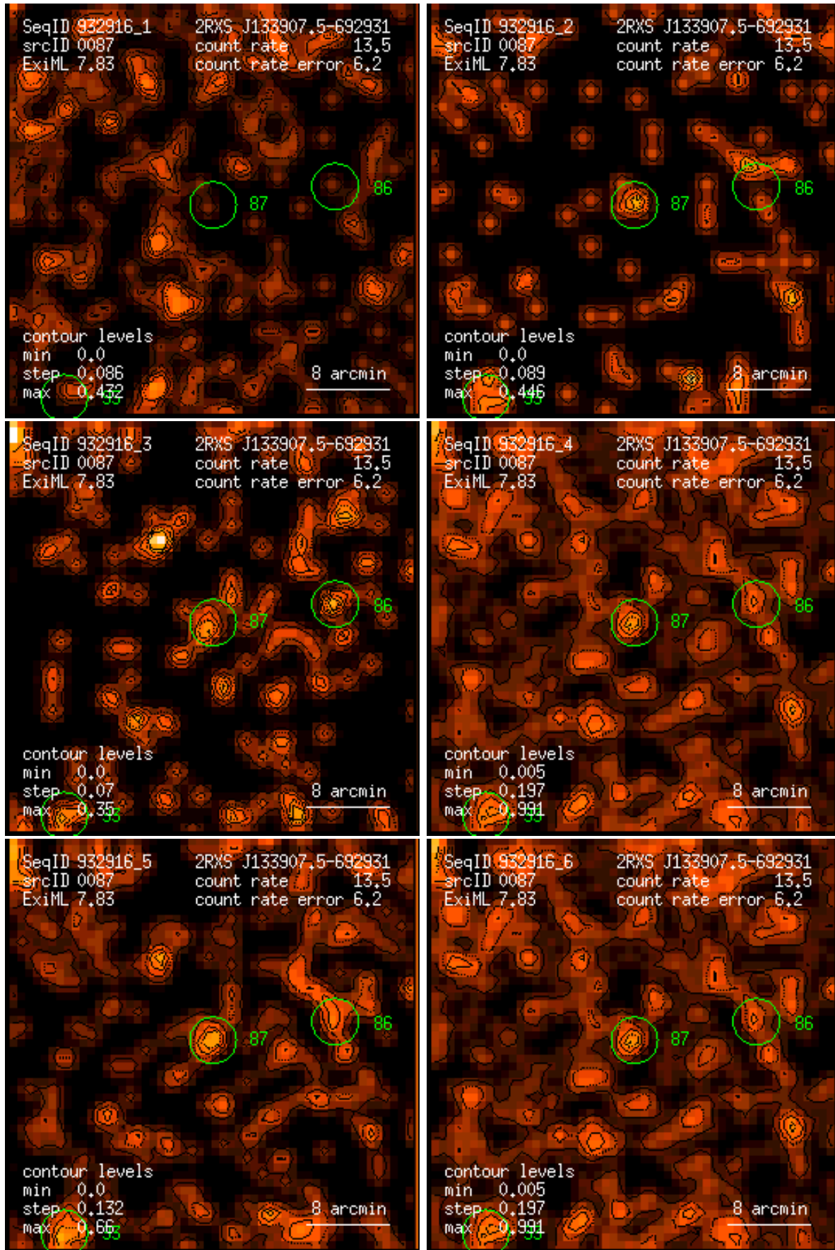
Figure 87: RASS 932916: detection 0087: band rate images, Gaussian filter: (1) PSPC channels 11 – 41, (2) 52 – 90, (3) 91 – 201, (4) 11 – 235, (5) 52 – 201, (6) 11 – 201. Broad band rates in counts/ks. Band rate contour levels in counts/ks/arcmin 2 .
