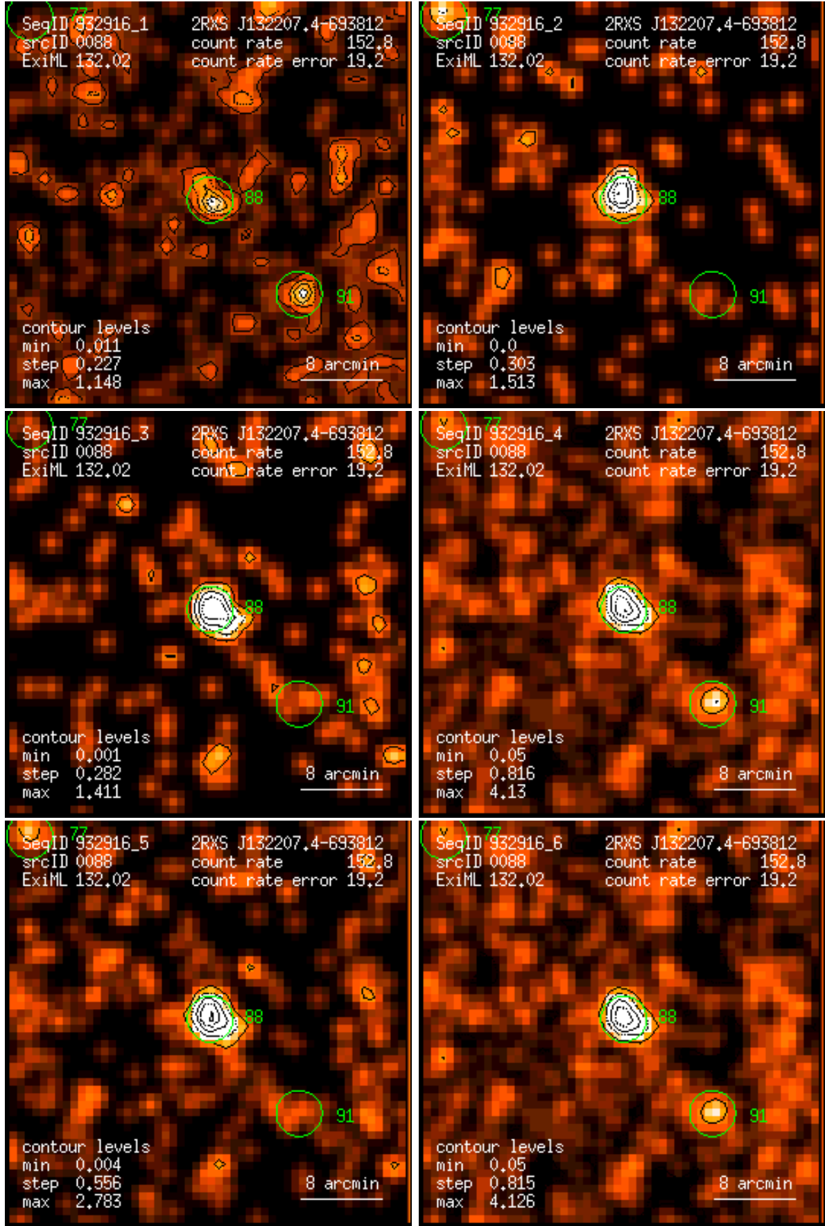
Figure 88: RASS 932916: detection 0088: band rate images, Gaussian filter: (1) PSPC channels 11 – 41, (2) 52 – 90, (3) 91 – 201, (4) 11 – 235, (5) 52 – 201, (6) 11 – 201. Broad band rates in counts/ks. Band rate contour levels in counts/ks/arcmin 2 .
