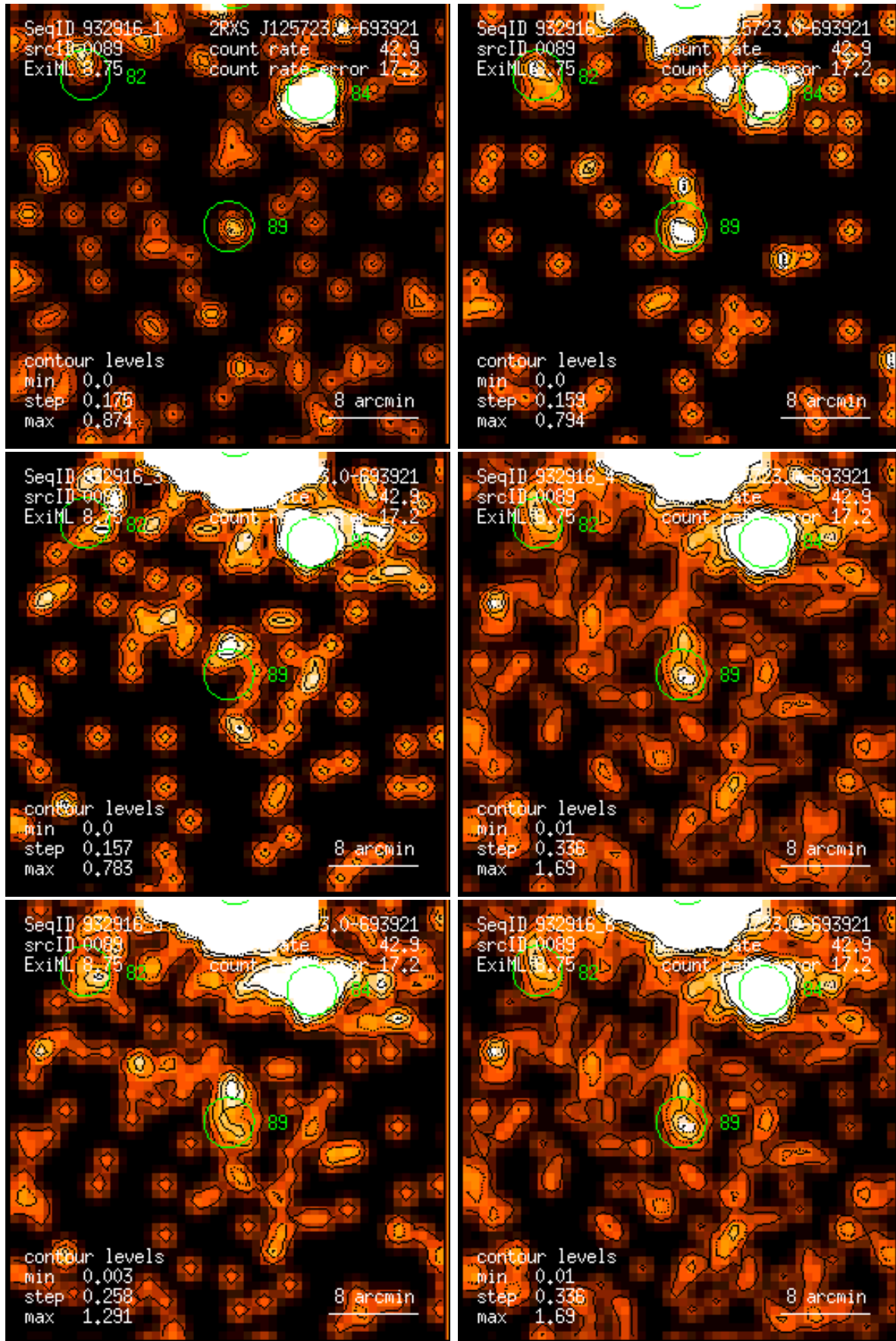
Figure 89: RASS 932916: detection 0089: band rate images, Gaussian filter: (1) PSPC channels 11 – 41, (2) 52 – 90, (3) 91 – 201, (4) 11 – 235, (5) 52 – 201, (6) 11 – 201. Broad band rates in counts/ks. Band rate contour levels in counts/ks/arcmin 2 .
