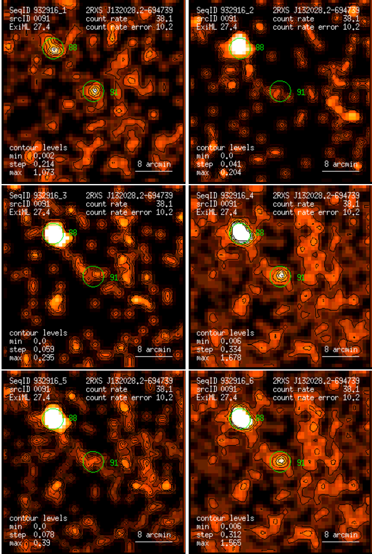
Figure 91: RASS 932916: detection 0091: band rate images, Gaussian filter: (1) PSPC channels 11 – 41, (2) 52 – 90, (3) 91 – 201, (4) 11 – 235, (5) 52 – 201, (6) 11 – 201. Broad band rates in counts/ks. Band rate contour levels in counts/ks/arcmin 2 .
