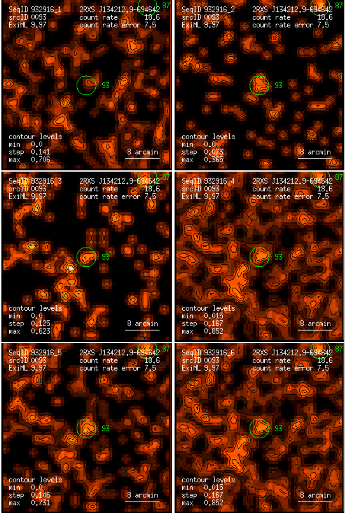
Figure 93: RASS 932916: detection 0093: band rate images, Gaussian filter: (1) PSPC channels 11 – 41, (2) 52 – 90, (3) 91 – 201, (4) 11 – 235, (5) 52 – 201, (6) 11 – 201. Broad band rates in counts/ks. Band rate contour levels in counts/ks/arcmin 2 .
