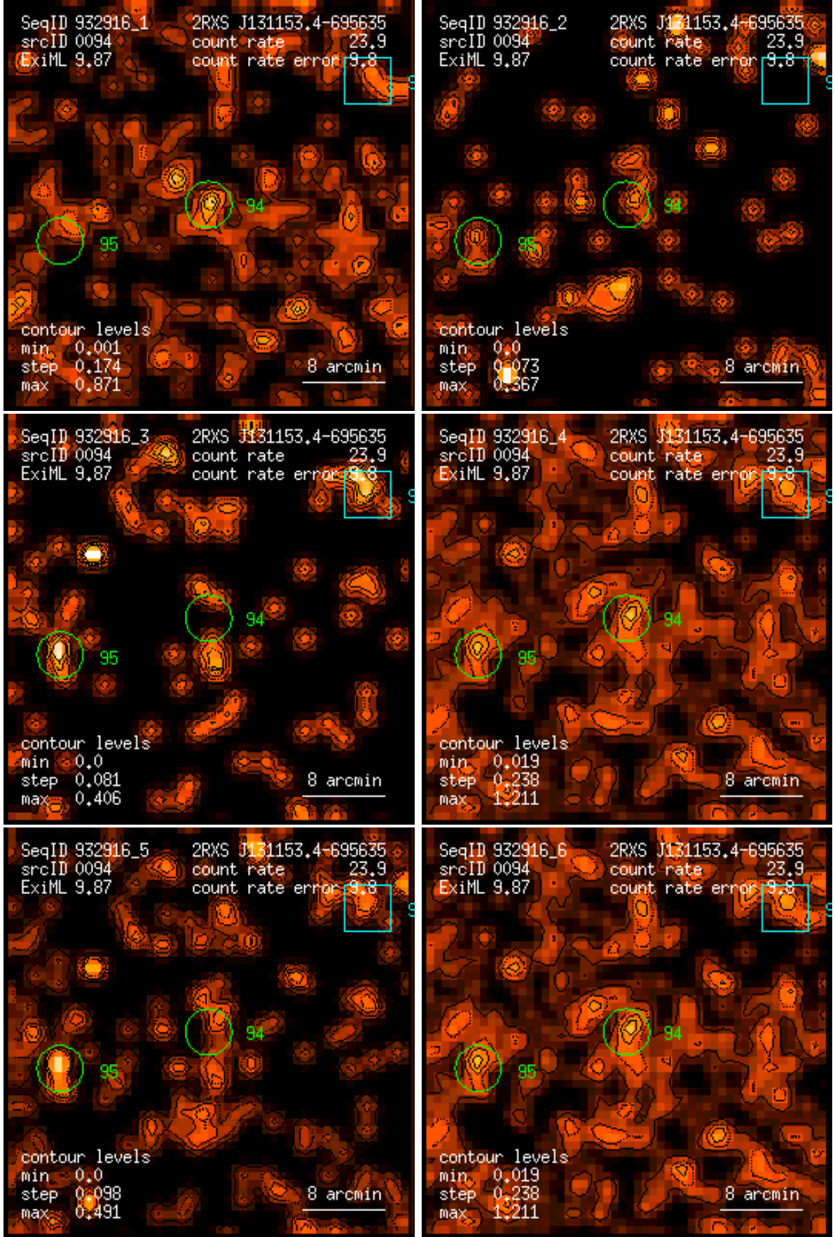
Figure 94: RASS 932916: detection 0094: band rate images, Gaussian filter: (1) PSPC channels 11 – 41, (2) 52 – 90, (3) 91 – 201, (4) 11 – 235, (5) 52 – 201, (6) 11 – 201. Broad band rates in counts/ks. Band rate contour levels in counts/ks/arcmin 2 .
