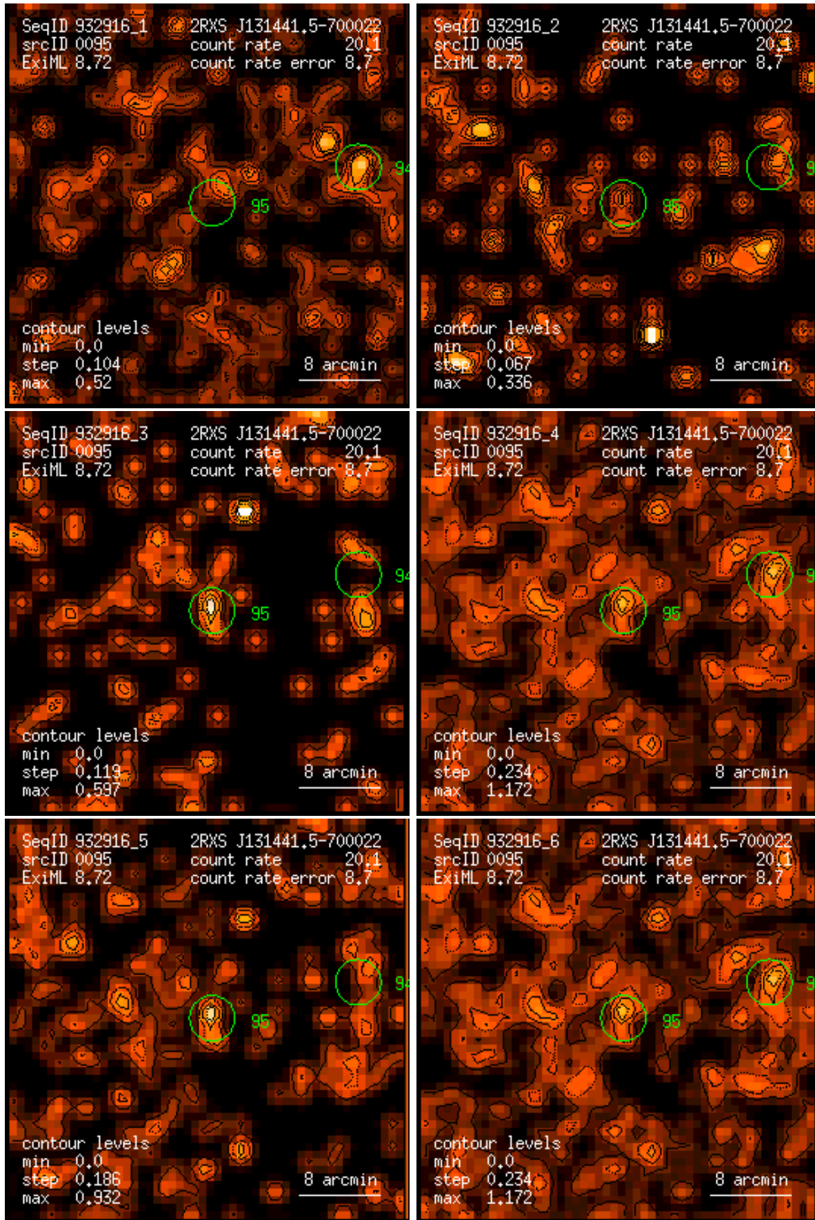
Figure 95: RASS 932916: detection 0095: band rate images, Gaussian filter: (1) PSPC channels 11 – 41, (2) 52 – 90, (3) 91 – 201, (4) 11 – 235, (5) 52 – 201, (6) 11 – 201. Broad band rates in counts/ks. Band rate contour levels in counts/ks/arcmin 2 .
