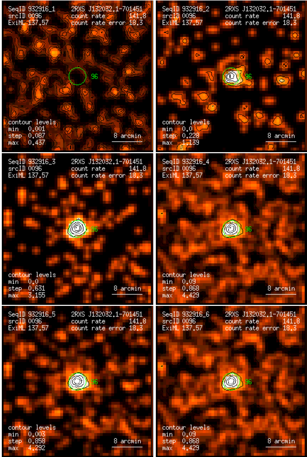
Figure 96: RASS 932916: detection 0096: band rate images, Gaussian filter: (1) PSPC channels 11 – 41, (2) 52 – 90, (3) 91 – 201, (4) 11 – 235, (5) 52 – 201, (6) 11 – 201. Broad band rates in counts/ks. Band rate contour levels in counts/ks/arcmin 2 .
