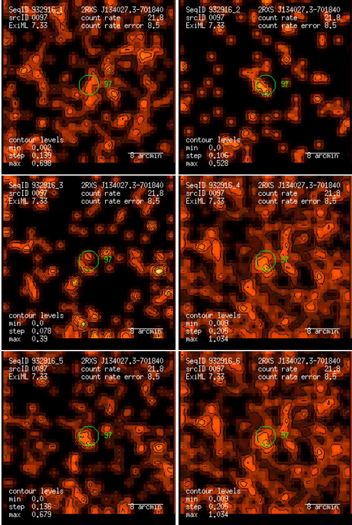
Figure 97: RASS 932916: detection 0097: band rate images, Gaussian filter: (1) PSPC channels 11 – 41, (2) 52 – 90, (3) 91 – 201, (4) 11 – 235, (5) 52 – 201, (6) 11 – 201. Broad band rates in counts/ks. Band rate contour levels in counts/ks/arcmin 2 .
