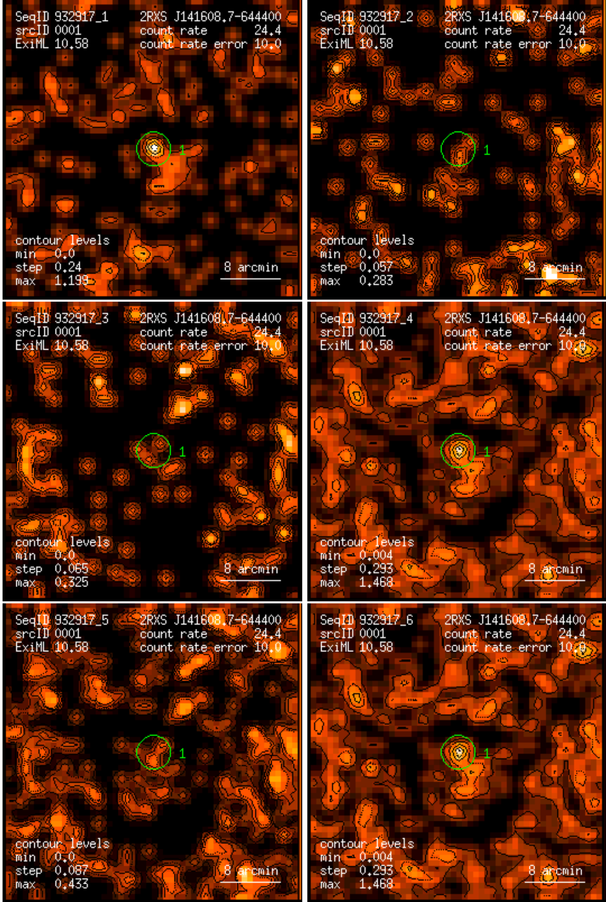
Figure 1: RASS 932917: detection 0001: band rate images, Gaussian filter: (1) PSPC channels 11 – 41, (2) 52 – 90, (3) 91 – 201, (4) 11 – 235, (5) 52 – 201, (6) 11 – 201. Broad band rates in counts/ks. Band rate contour levels in counts/ks/arcmin 2 .
