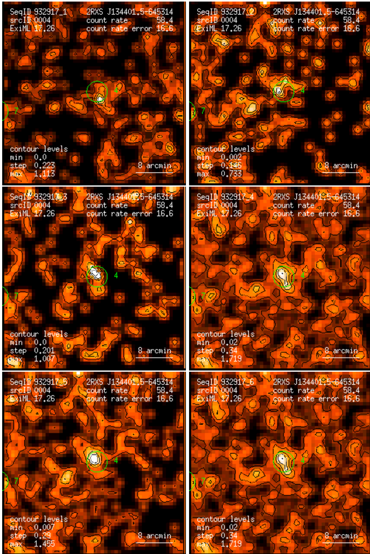
Figure 4: RASS 932917: detection 0004: band rate images, Gaussian filter: (1) PSPC channels 11 – 41, (2) 52 – 90, (3) 91 – 201, (4) 11 – 235, (5) 52 – 201, (6) 11 – 201. Broad band rates in counts/ks. Band rate contour levels in counts/ks/arcmin 2 .
