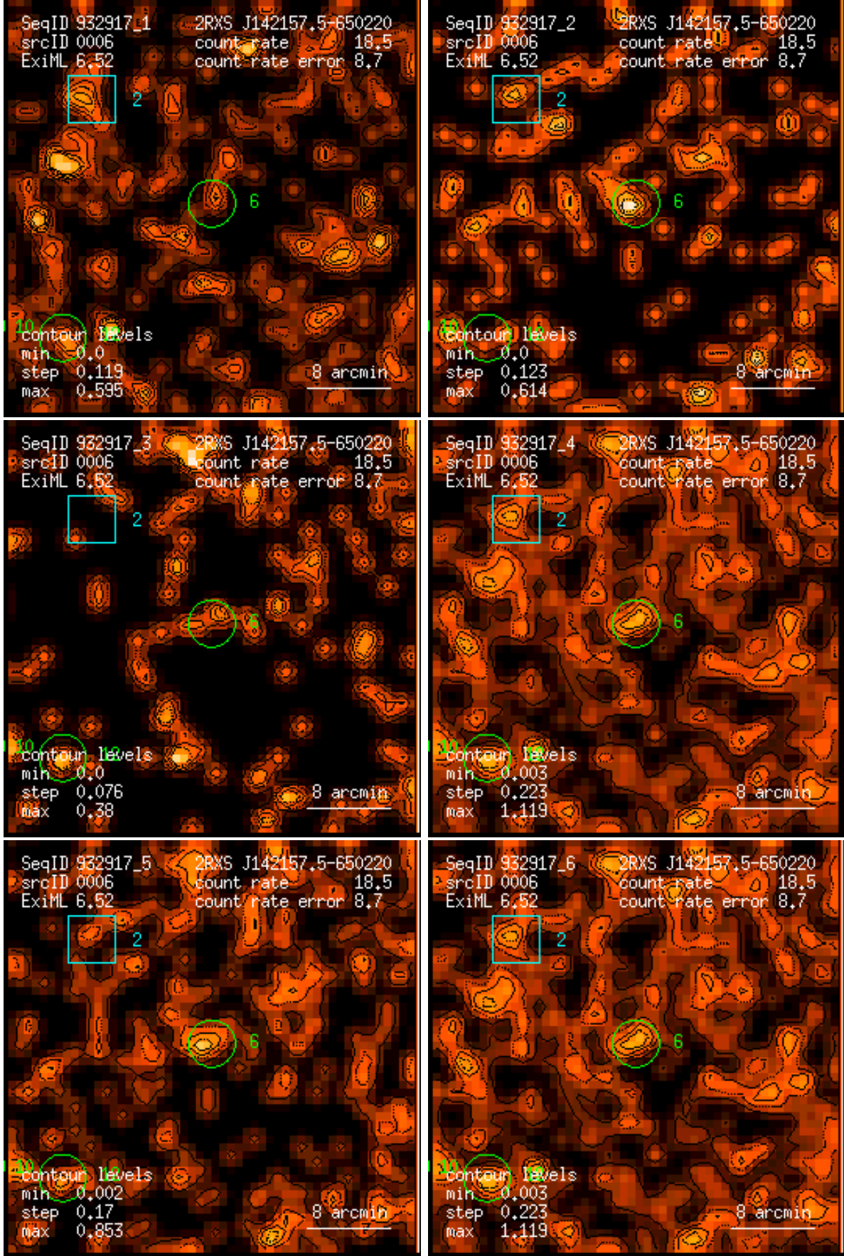
Figure 6: RASS 932917: detection 0006: band rate images, Gaussian filter: (1) PSPC channels 11 – 41, (2) 52 – 90, (3) 91 – 201, (4) 11 – 235, (5) 52 – 201, (6) 11 – 201. Broad band rates in counts/ks. Band rate contour levels in counts/ks/arcmin 2 .
