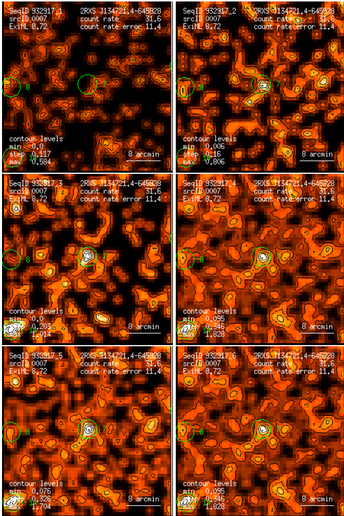
Figure 7: RASS 932917: detection 0007: band rate images, Gaussian filter: (1) PSPC channels 11 – 41, (2) 52 – 90, (3) 91 – 201, (4) 11 – 235, (5) 52 – 201, (6) 11 – 201. Broad band rates in counts/ks. Band rate contour levels in counts/ks/arcmin 2 .
