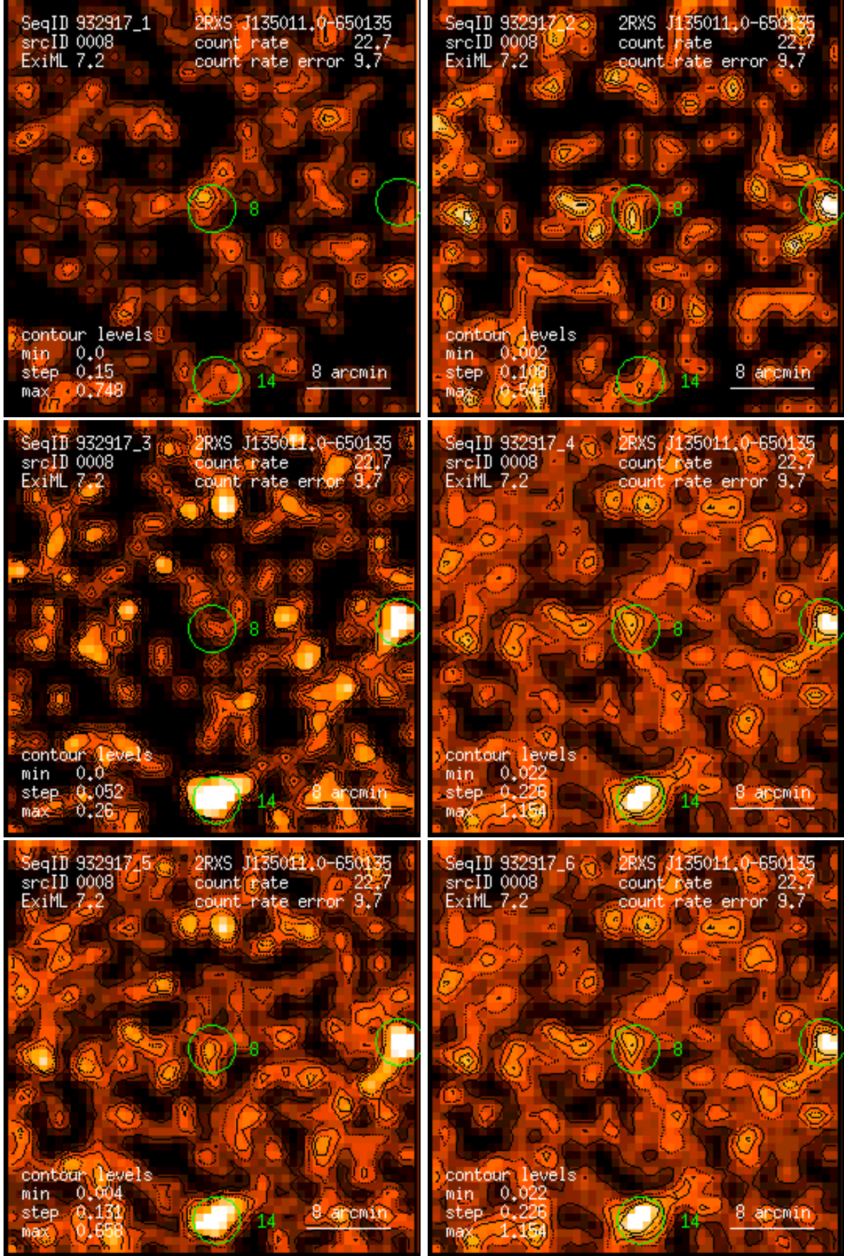
Figure 8: RASS 932917: detection 0008: band rate images, Gaussian filter: (1) PSPC channels 11 – 41, (2) 52 – 90, (3) 91 – 201, (4) 11 – 235, (5) 52 – 201, (6) 11 – 201. Broad band rates in counts/ks. Band rate contour levels in counts/ks/arcmin 2 .
