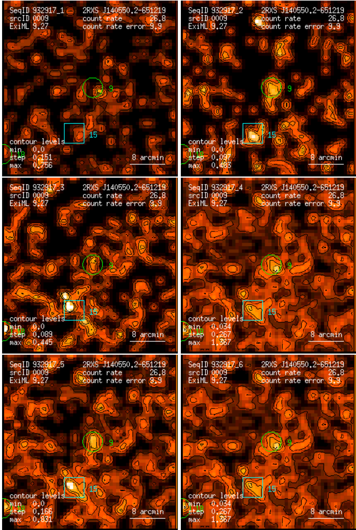
Figure 9: RASS 932917: detection 0009: band rate images, Gaussian filter: (1) PSPC channels 11 – 41, (2) 52 – 90, (3) 91 – 201, (4) 11 – 235, (5) 52 – 201, (6) 11 – 201. Broad band rates in counts/ks. Band rate contour levels in counts/ks/arcmin 2 .
