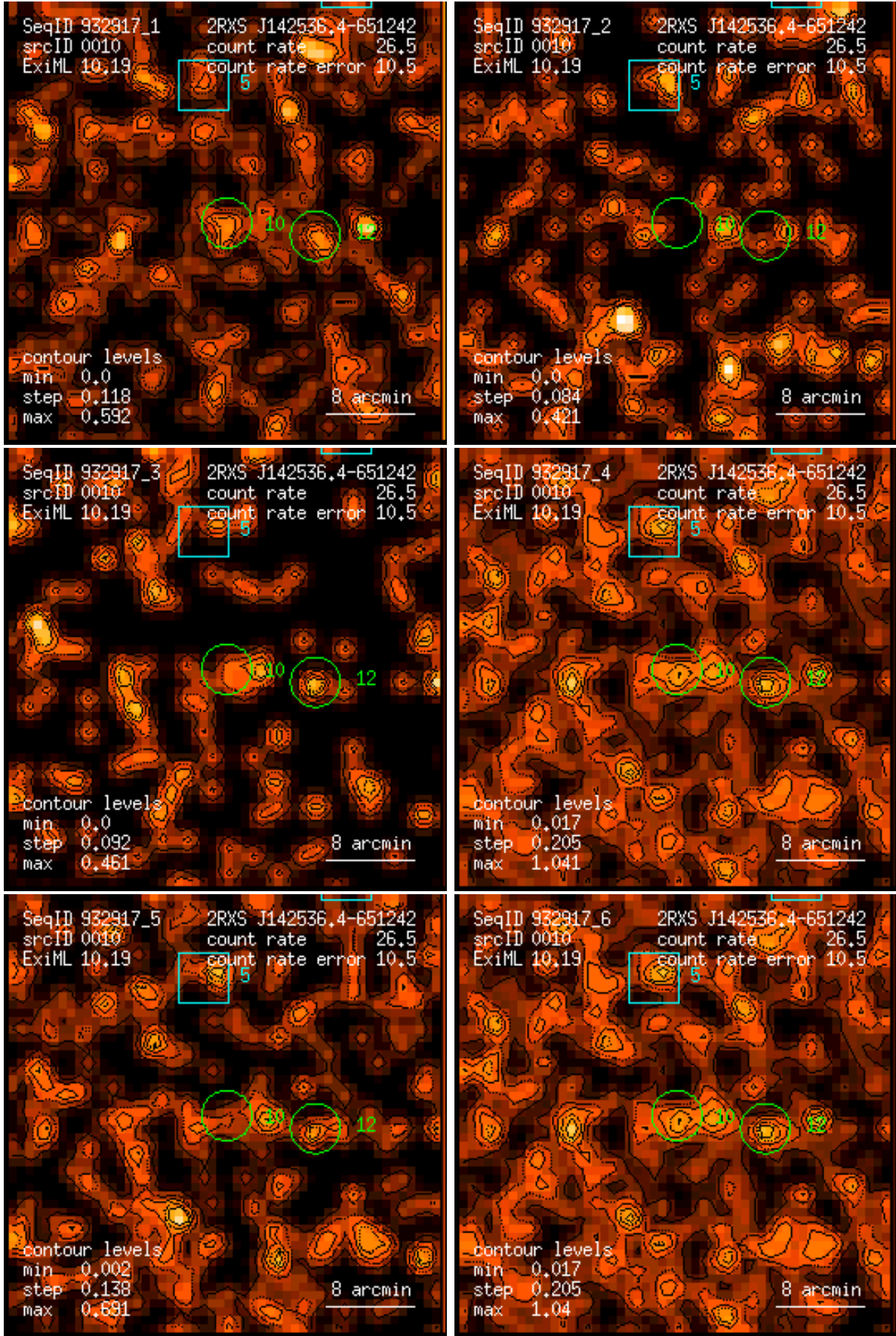
Figure 10: RASS 932917: detection 0010: band rate images, Gaussian filter: (1) PSPC channels 11 – 41, (2) 52 – 90, (3) 91 – 201, (4) 11 – 235, (5) 52 – 201, (6) 11 – 201. Broad band rates in counts/ks. Band rate contour levels in counts/ks/arcmin 2 .
