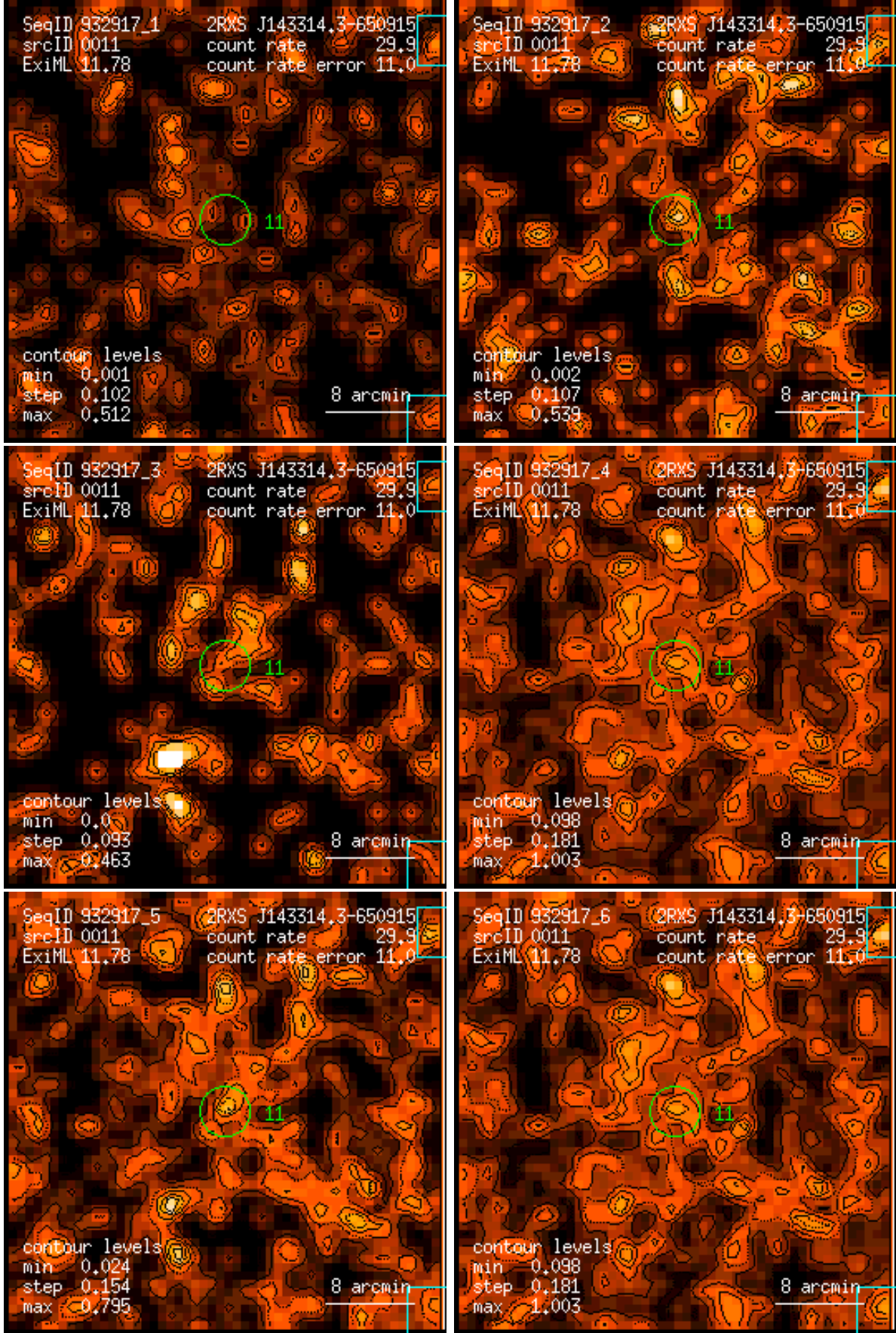
Figure 11: RASS 932917: detection 0011: band rate images, Gaussian filter: (1) PSPC channels 11 – 41, (2) 52 – 90, (3) 91 – 201, (4) 11 – 235, (5) 52 – 201, (6) 11 – 201. Broad band rates in counts/ks. Band rate contour levels in counts/ks/arcmin 2 .
