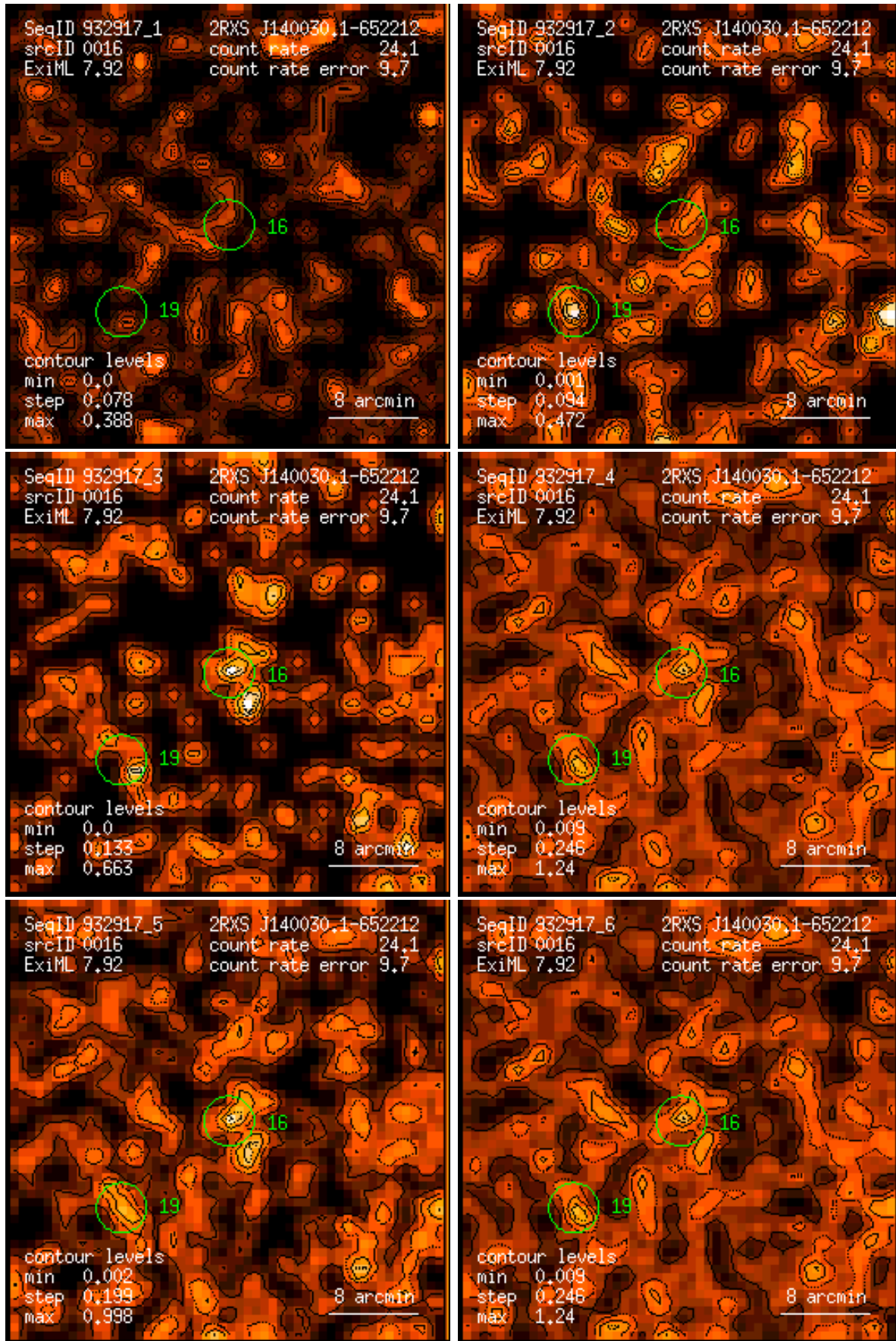
Figure 16: RASS 932917: detection 0016: band rate images, Gaussian filter: (1) PSPC channels 11 – 41, (2) 52 – 90, (3) 91 – 201, (4) 11 – 235, (5) 52 – 201, (6) 11 – 201. Broad band rates in counts/ks. Band rate contour levels in counts/ks/arcmin 2 .
