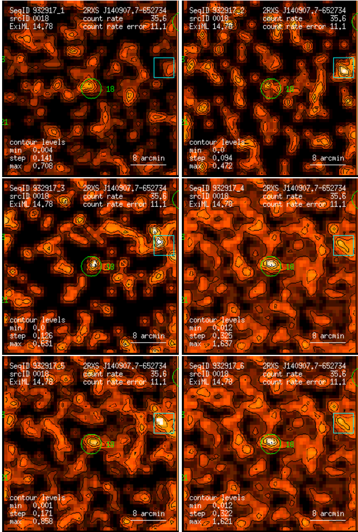
Figure 18: RASS 932917: detection 0018: band rate images, Gaussian filter: (1) PSPC channels 11 – 41, (2) 52 – 90, (3) 91 – 201, (4) 11 – 235, (5) 52 – 201, (6) 11 – 201. Broad band rates in counts/ks. Band rate contour levels in counts/ks/arcmin 2 .
