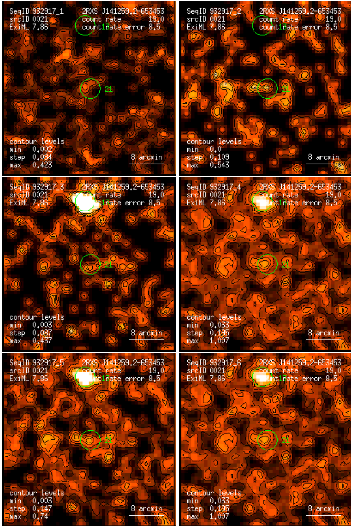
Figure 21: RASS 932917: detection 0021: band rate images, Gaussian filter: (1) PSPC channels 11 – 41, (2) 52 – 90, (3) 91 – 201, (4) 11 – 235, (5) 52 – 201, (6) 11 – 201. Broad band rates in counts/ks. Band rate contour levels in counts/ks/arcmin 2 .
