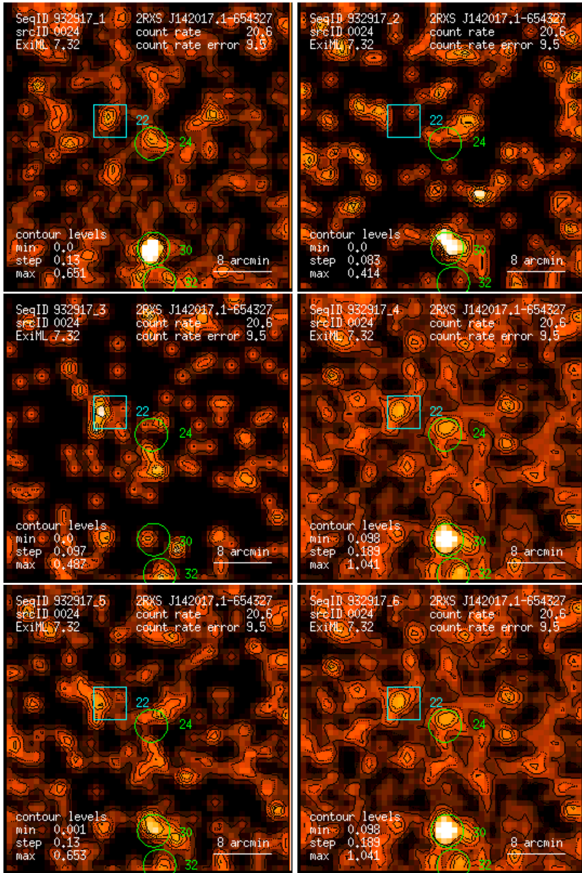
Figure 24: RASS 932917: detection 0024: band rate images, Gaussian filter: (1) PSPC channels 11 – 41, (2) 52 – 90, (3) 91 – 201, (4) 11 – 235, (5) 52 – 201, (6) 11 – 201. Broad band rates in counts/ks. Band rate contour levels in counts/ks/arcmin 2 .
