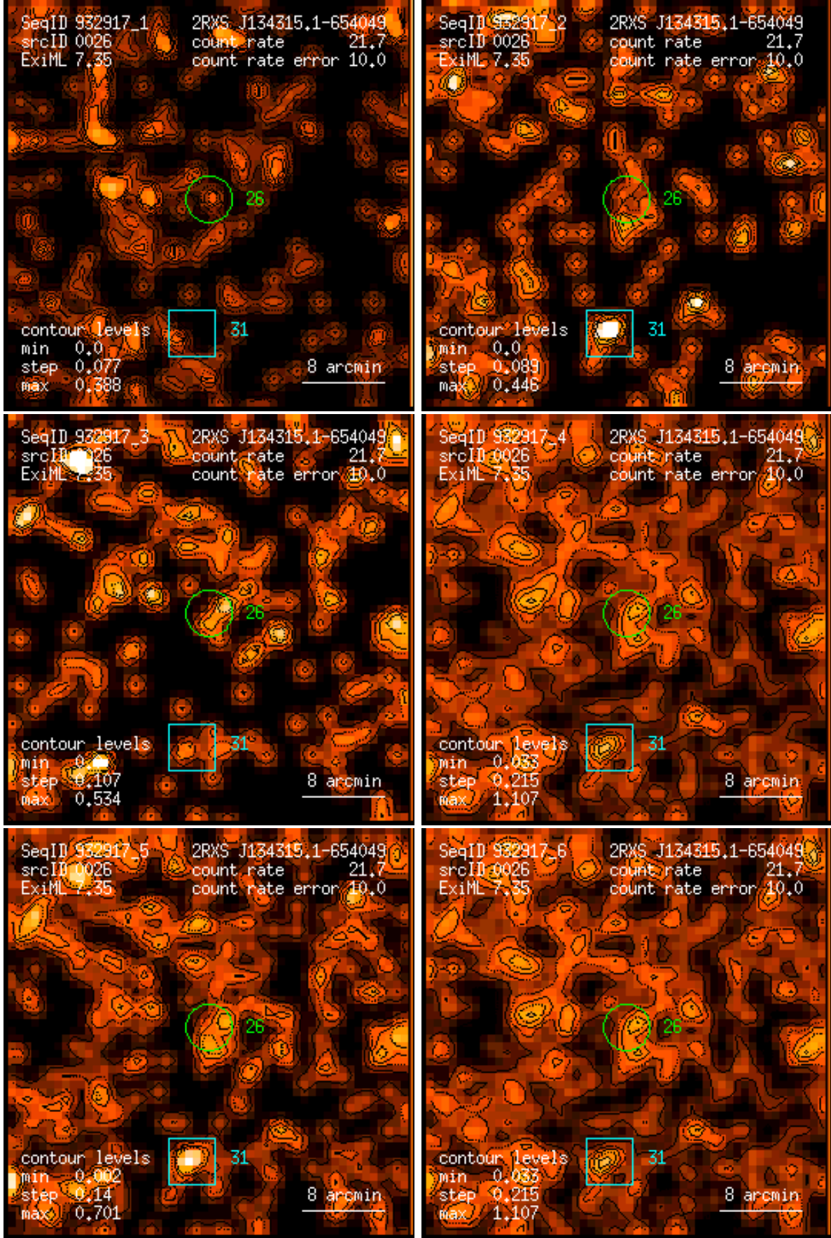
Figure 26: RASS 932917: detection 0026: band rate images, Gaussian filter: (1) PSPC channels 11 – 41, (2) 52 – 90, (3) 91 – 201, (4) 11 – 235, (5) 52 – 201, (6) 11 – 201. Broad band rates in counts/ks. Band rate contour levels in counts/ks/arcmin 2 .
