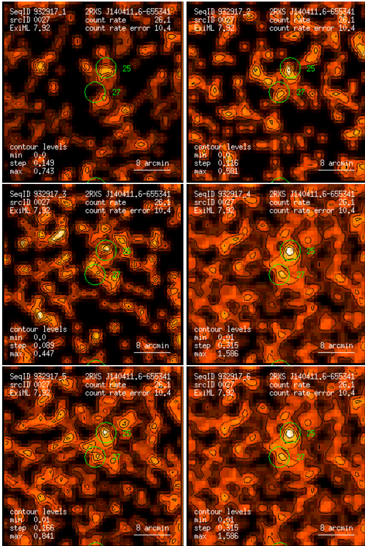
Figure 27: RASS 932917: detection 0027: band rate images, Gaussian filter: (1) PSPC channels 11 – 41, (2) 52 – 90, (3) 91 – 201, (4) 11 – 235, (5) 52 – 201, (6) 11 – 201. Broad band rates in counts/ks. Band rate contour levels in counts/ks/arcmin 2 .
