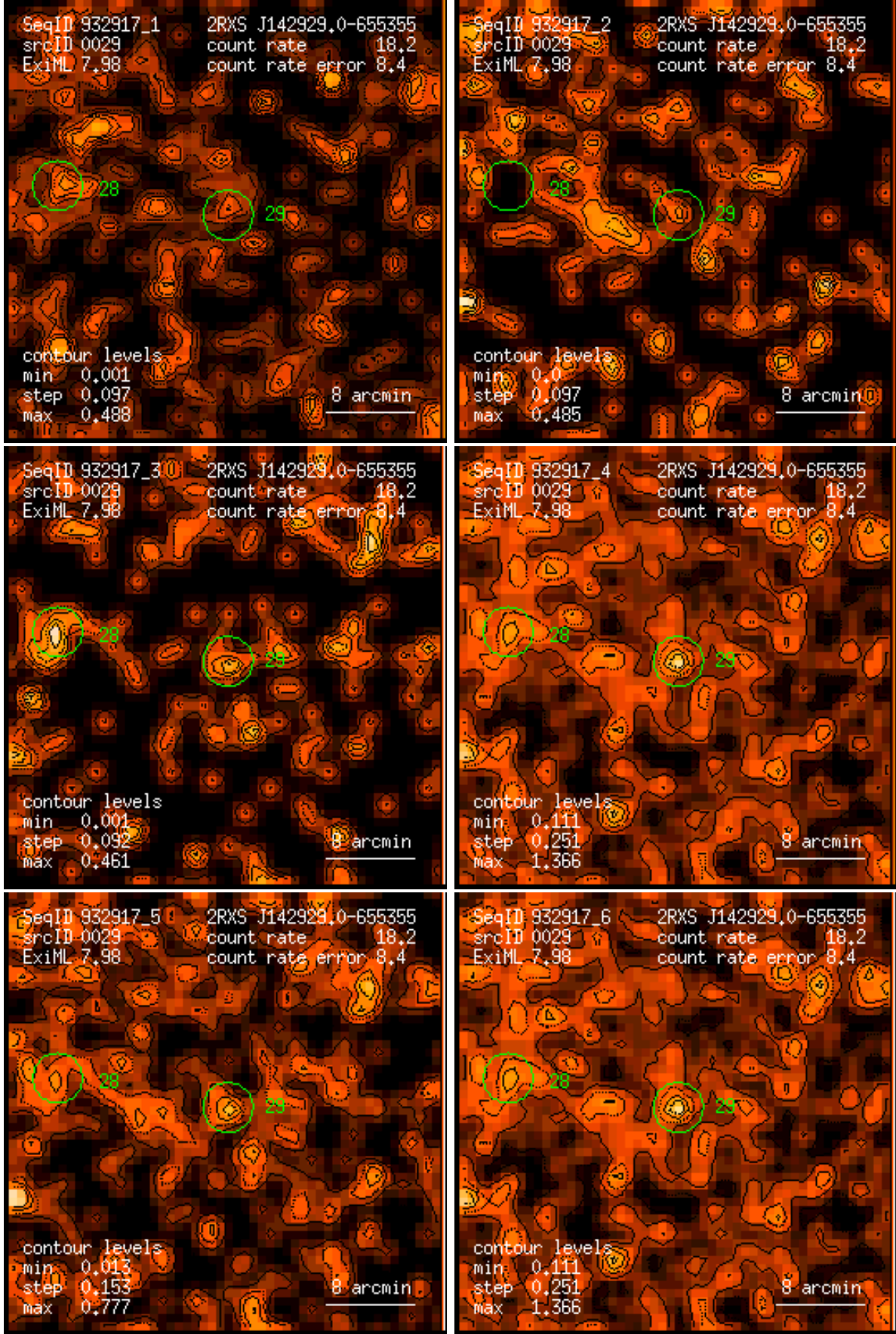
Figure 29: RASS 932917: detection 0029: band rate images, Gaussian filter: (1) PSPC channels 11 – 41, (2) 52 – 90, (3) 91 – 201, (4) 11 – 235, (5) 52 – 201, (6) 11 – 201. Broad band rates in counts/ks. Band rate contour levels in counts/ks/arcmin 2 .
