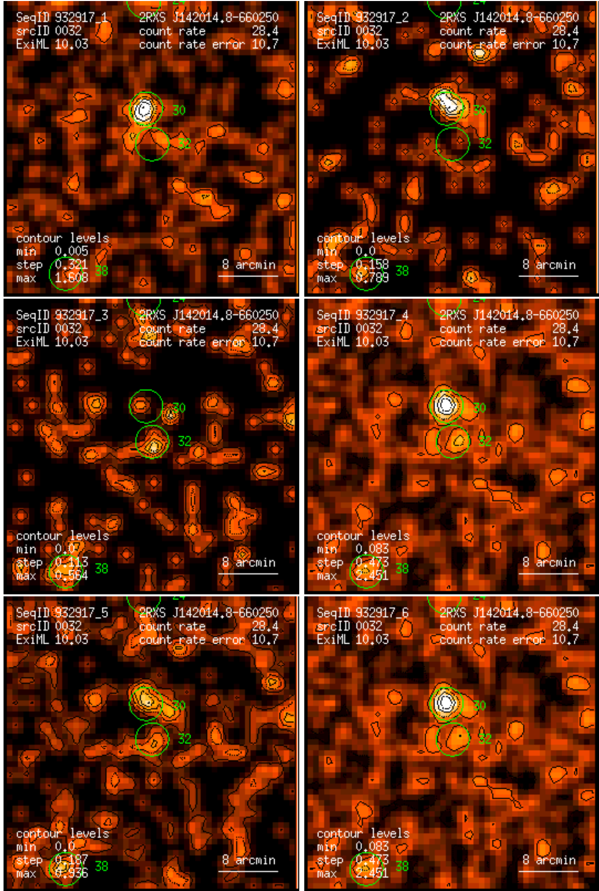
Figure 32: RASS 932917: detection 0032: band rate images, Gaussian filter: (1) PSPC channels 11 – 41, (2) 52 – 90, (3) 91 – 201, (4) 11 – 235, (5) 52 – 201, (6) 11 – 201. Broad band rates in counts/ks. Band rate contour levels in counts/ks/arcmin 2 .
