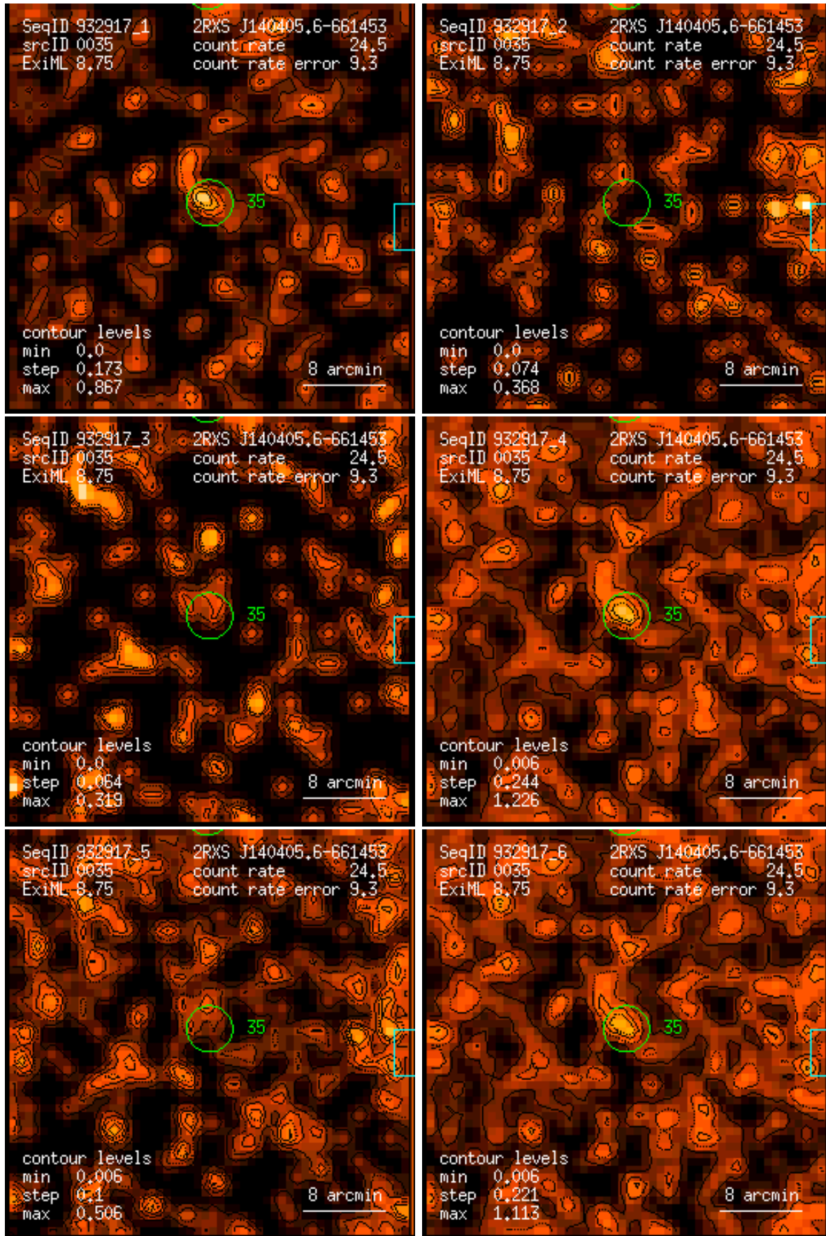
Figure 35: RASS 932917: detection 0035: band rate images, Gaussian filter: (1) PSPC channels 11 – 41, (2) 52 – 90, (3) 91 – 201, (4) 11 – 235, (5) 52 – 201, (6) 11 – 201. Broad band rates in counts/ks. Band rate contour levels in counts/ks/arcmin 2 .
