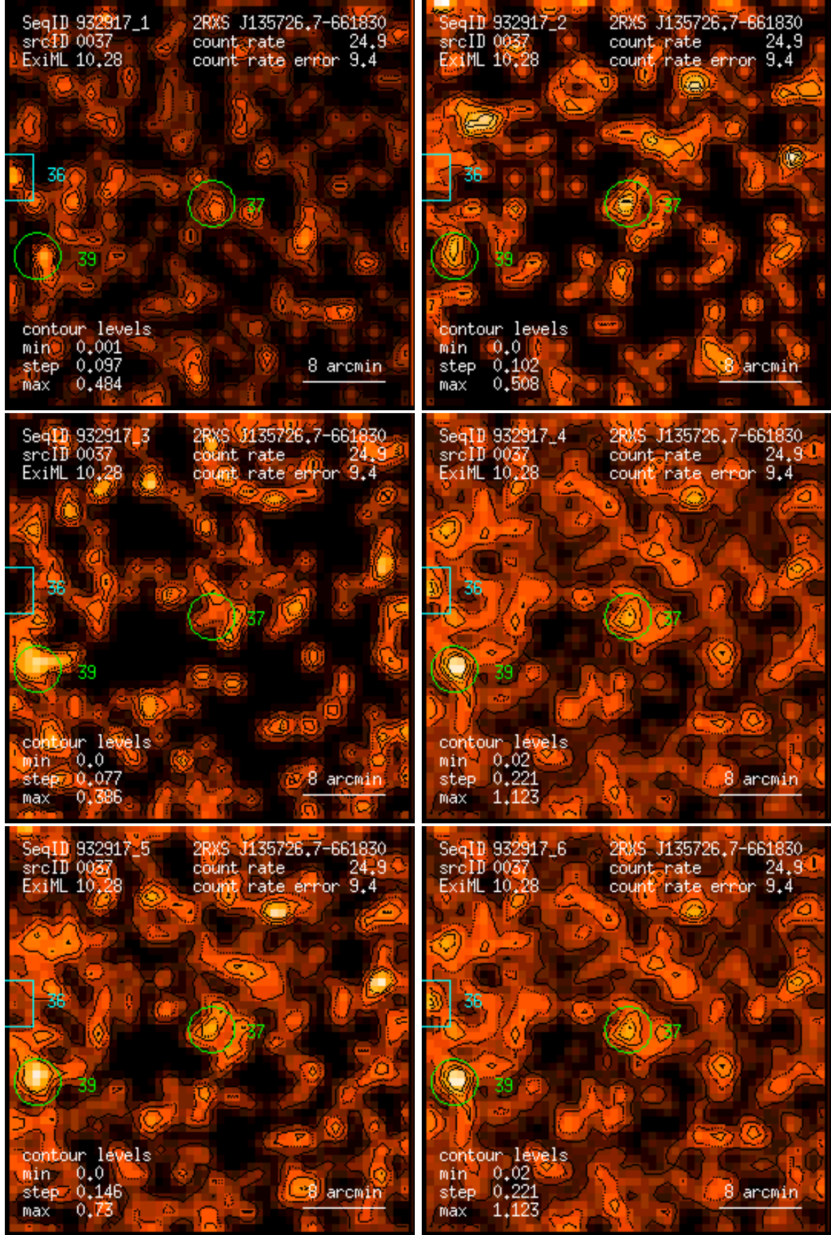
Figure 37: RASS 932917: detection 0037: band rate images, Gaussian filter: (1) PSPC channels 11 – 41, (2) 52 – 90, (3) 91 – 201, (4) 11 – 235, (5) 52 – 201, (6) 11 – 201. Broad band rates in counts/ks. Band rate contour levels in counts/ks/arcmin 2 .
