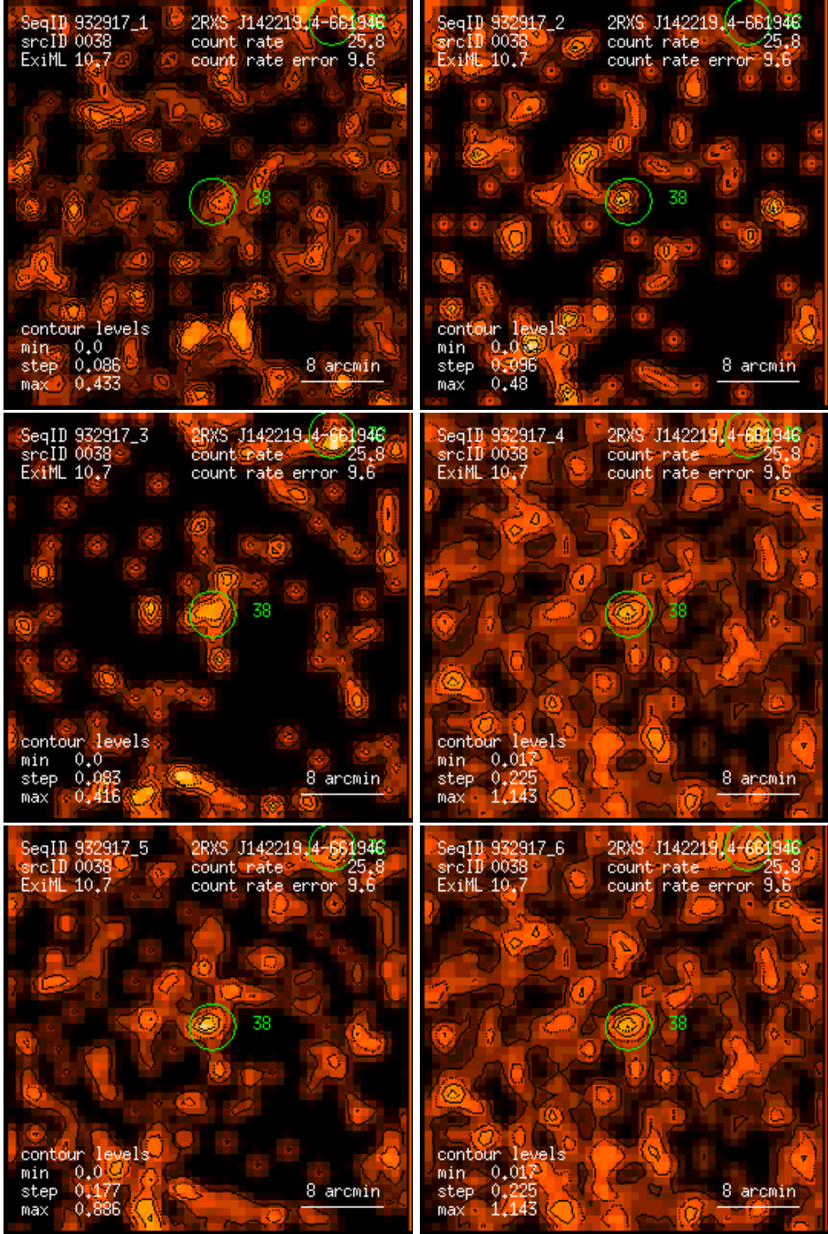
Figure 38: RASS 932917: detection 0038: band rate images, Gaussian filter: (1) PSPC channels 11 – 41, (2) 52 – 90, (3) 91 – 201, (4) 11 – 235, (5) 52 – 201, (6) 11 – 201. Broad band rates in counts/ks. Band rate contour levels in counts/ks/arcmin 2 .
