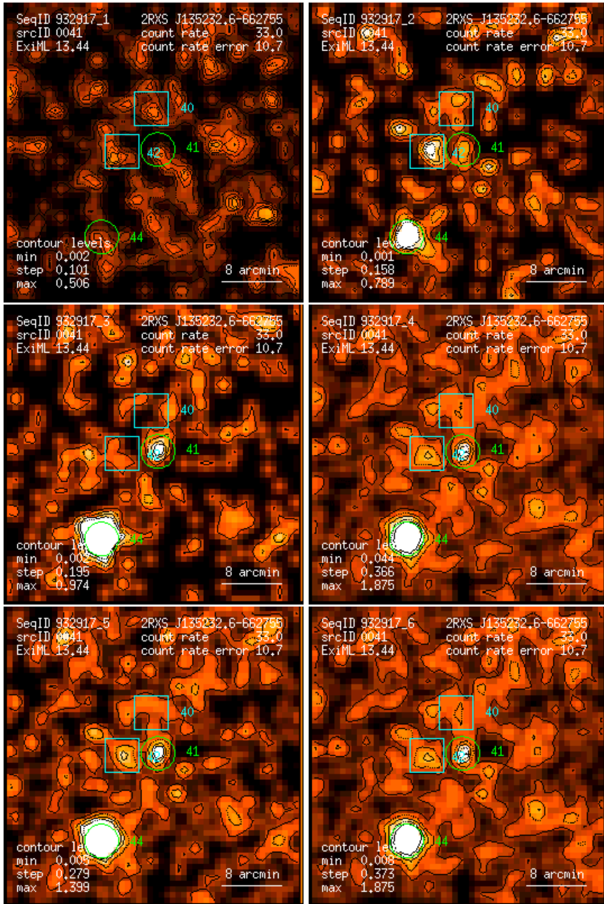
Figure 41: RASS 932917: detection 0041: band rate images, Gaussian filter: (1) PSPC channels 11 – 41, (2) 52 – 90, (3) 91 – 201, (4) 11 – 235, (5) 52 – 201, (6) 11 – 201. Broad band rates in counts/ks. Band rate contour levels in counts/ks/arcmin 2 .
