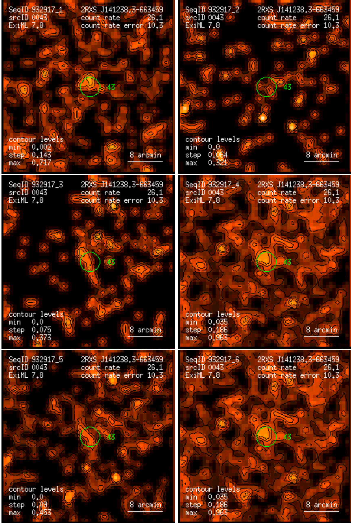
Figure 43: RASS 932917: detection 0043: band rate images, Gaussian filter: (1) PSPC channels 11 – 41, (2) 52 – 90, (3) 91 – 201, (4) 11 – 235, (5) 52 – 201, (6) 11 – 201. Broad band rates in counts/ks. Band rate contour levels in counts/ks/arcmin 2 .
