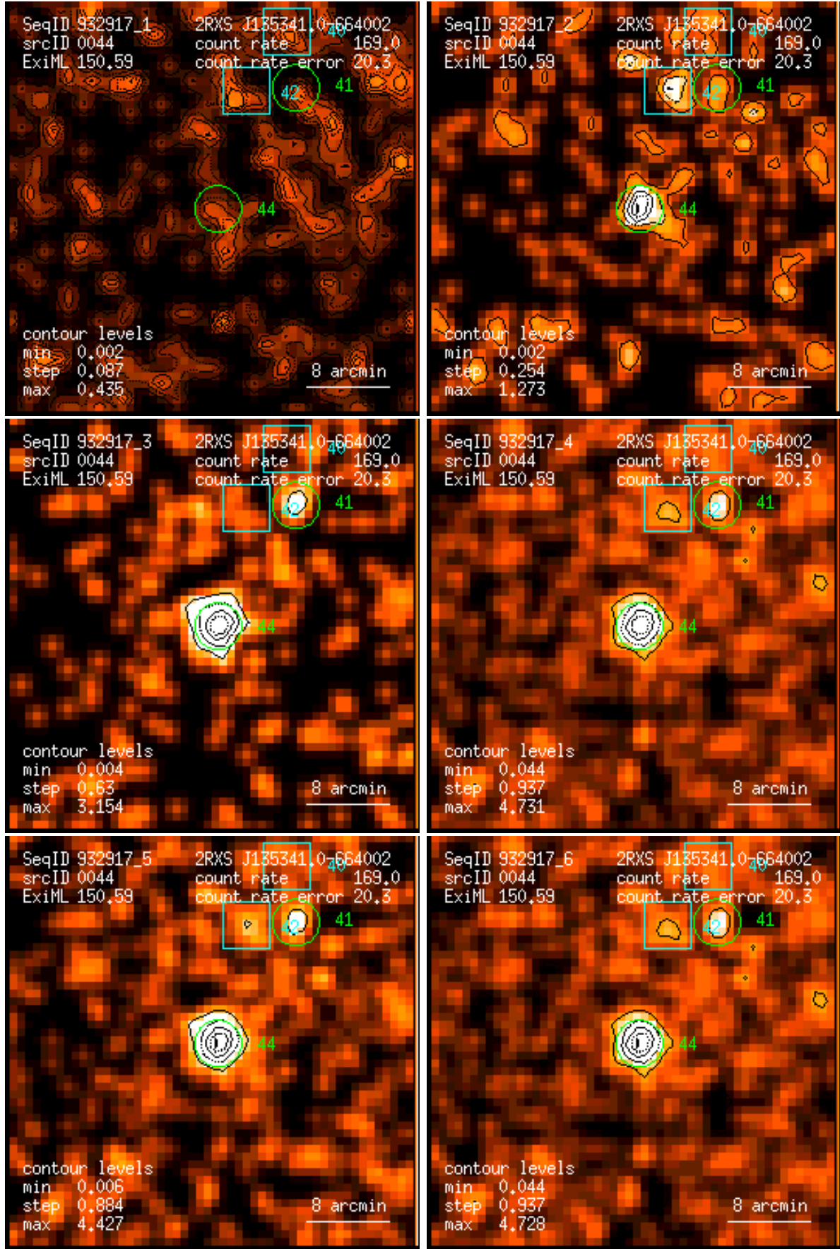
Figure 44: RASS 932917: detection 0044: band rate images, Gaussian filter: (1) PSPC channels 11 – 41, (2) 52 – 90, (3) 91 – 201, (4) 11 – 235, (5) 52 – 201, (6) 11 – 201. Broad band rates in counts/ks. Band rate contour levels in counts/ks/arcmin 2 .
