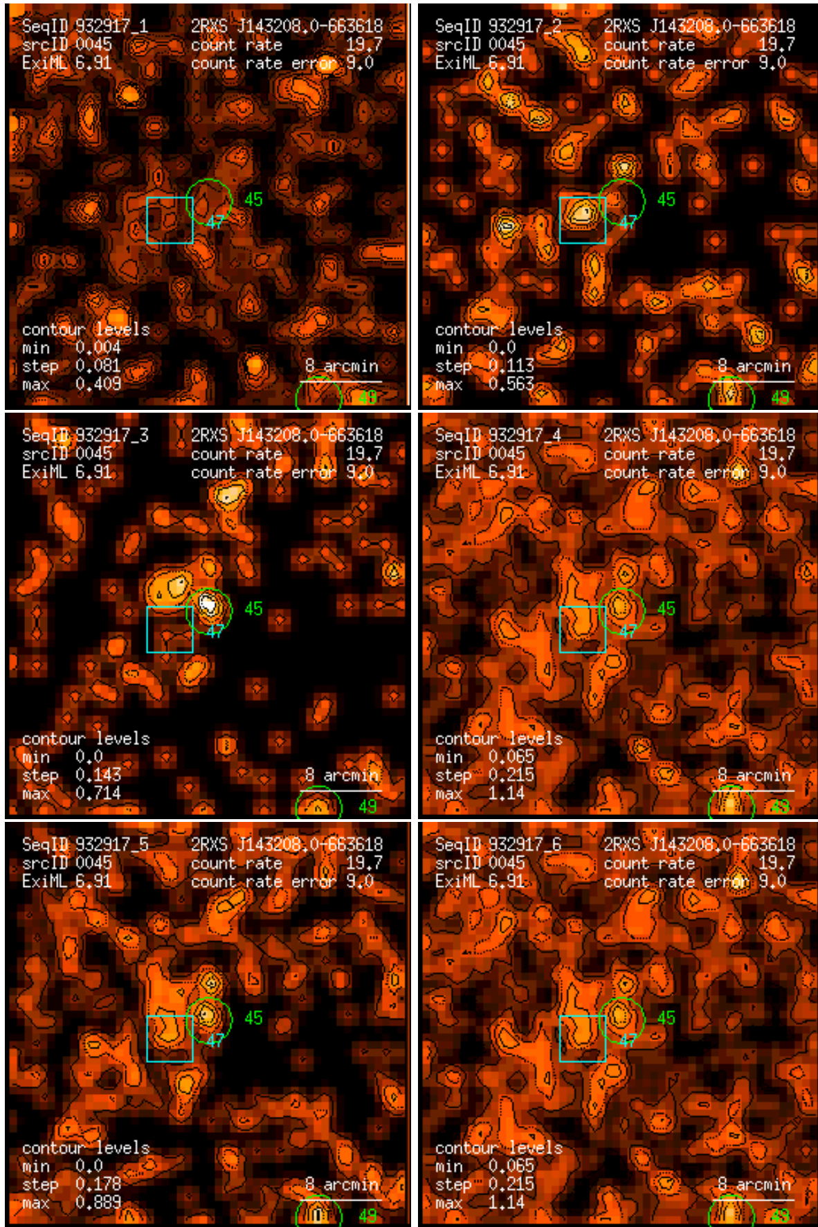
Figure 45: RASS 932917: detection 0045: band rate images, Gaussian filter: (1) PSPC channels 11 – 41, (2) 52 – 90, (3) 91 – 201, (4) 11 – 235, (5) 52 – 201, (6) 11 – 201. Broad band rates in counts/ks. Band rate contour levels in counts/ks/arcmin 2 .
