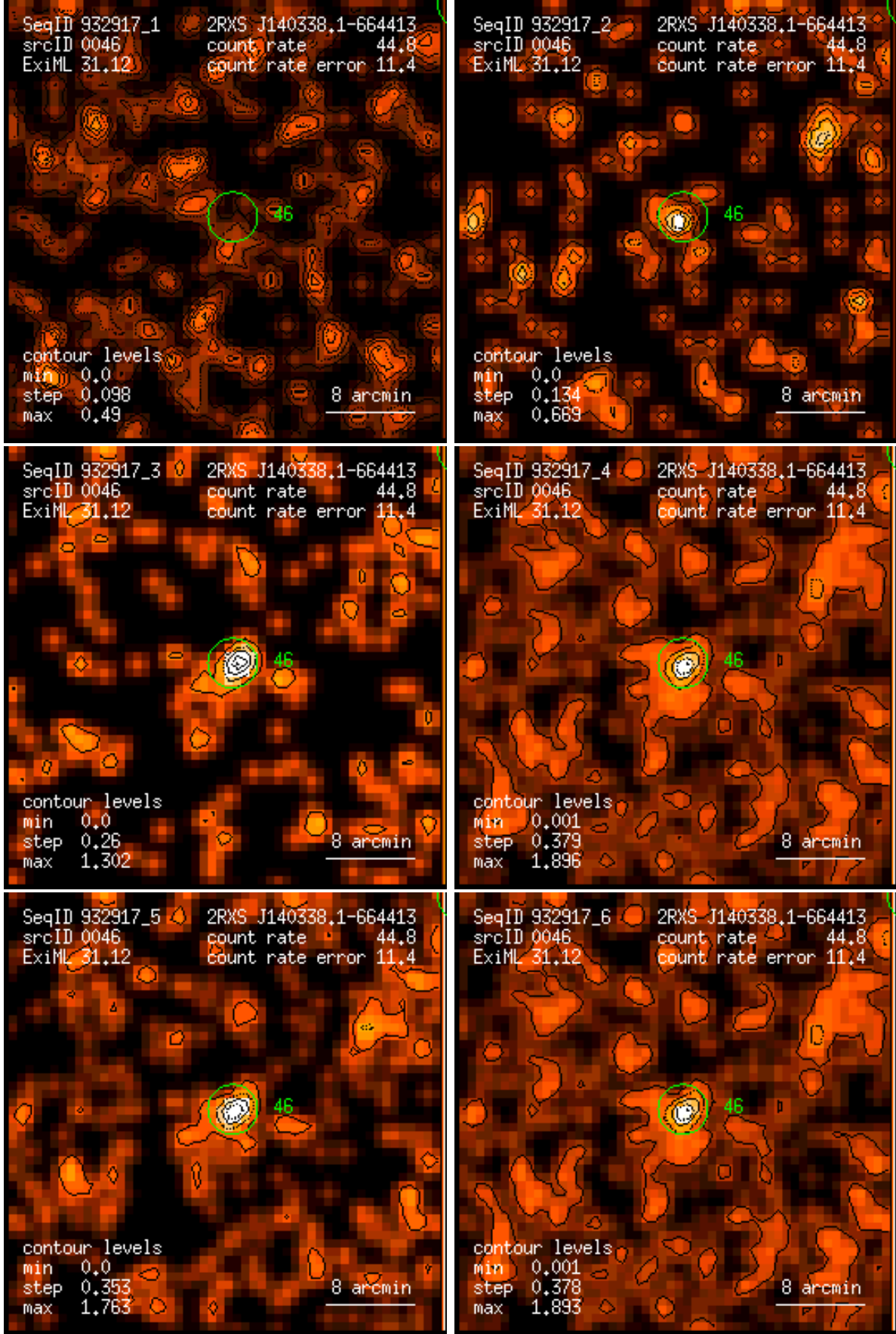
Figure 46: RASS 932917: detection 0046: band rate images, Gaussian filter: (1) PSPC channels 11 – 41, (2) 52 – 90, (3) 91 – 201, (4) 11 – 235, (5) 52 – 201, (6) 11 – 201. Broad band rates in counts/ks. Band rate contour levels in counts/ks/arcmin 2 .
