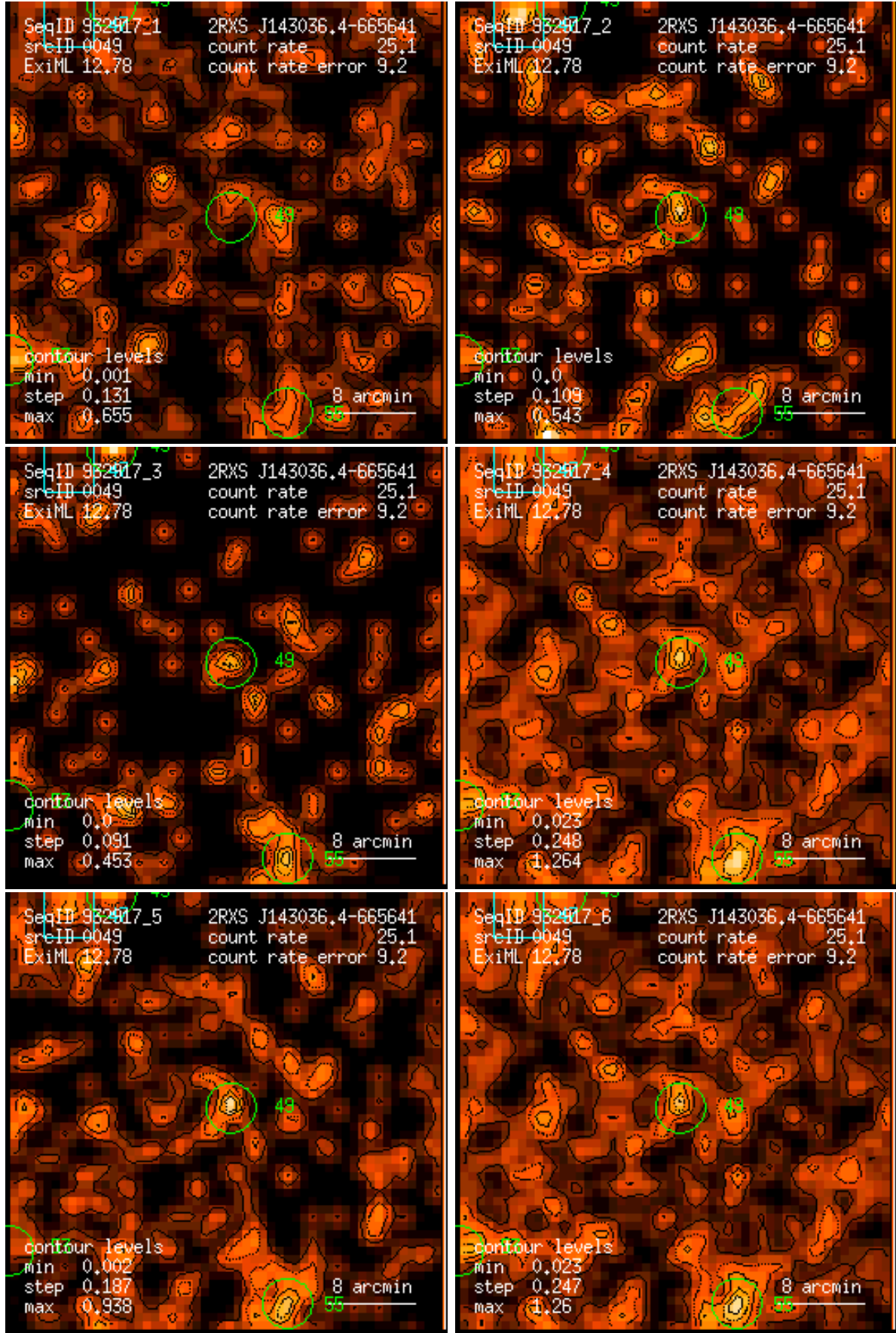
Figure 49: RASS 932917: detection 0049: band rate images, Gaussian filter: (1) PSPC channels 11 – 41, (2) 52 – 90, (3) 91 – 201, (4) 11 – 235, (5) 52 – 201, (6) 11 – 201. Broad band rates in counts/ks. Band rate contour levels in counts/ks/arcmin 2 .
