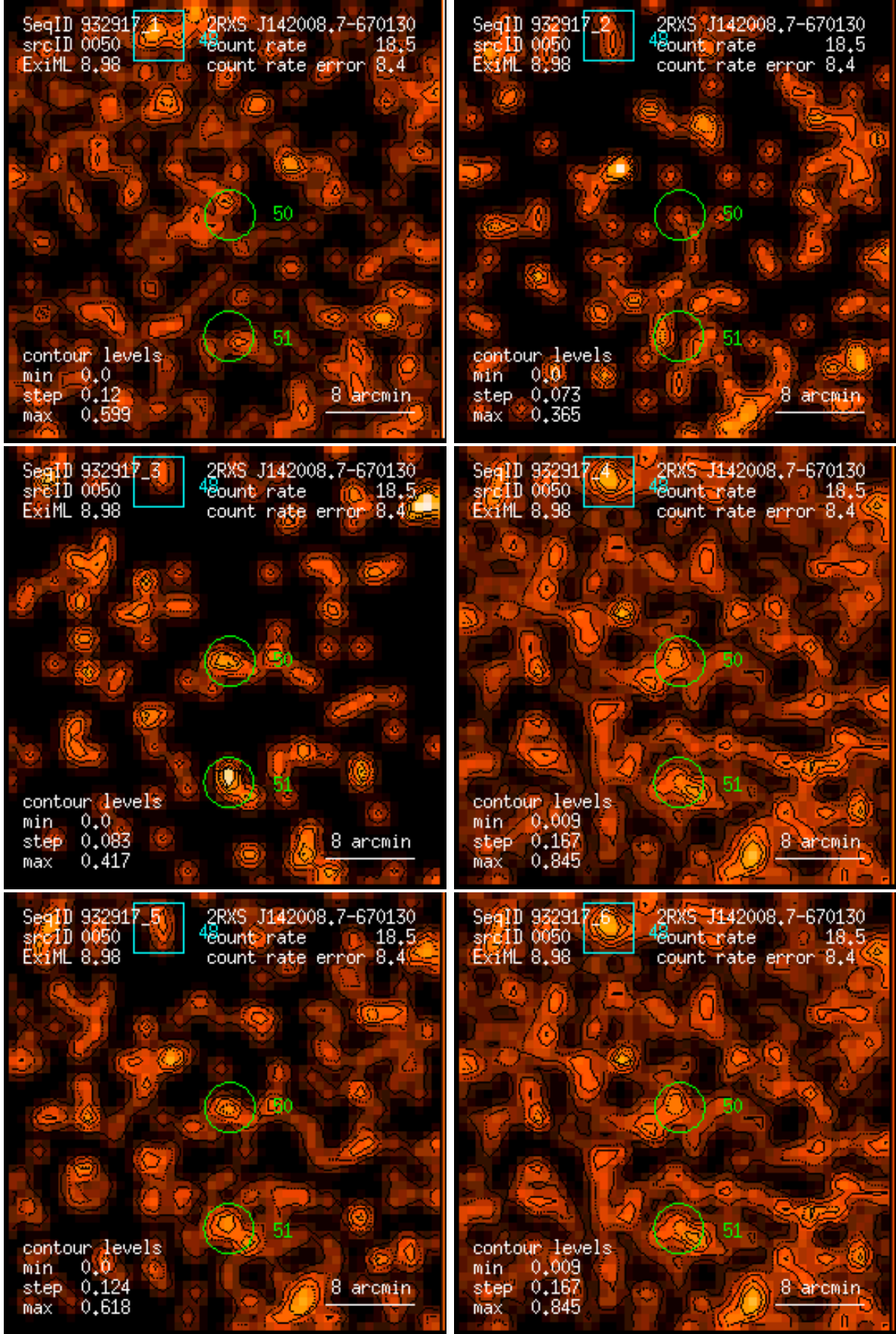
Figure 50: RASS 932917: detection 0050: band rate images, Gaussian filter: (1) PSPC channels 11 – 41, (2) 52 – 90, (3) 91 – 201, (4) 11 – 235, (5) 52 – 201, (6) 11 – 201. Broad band rates in counts/ks. Band rate contour levels in counts/ks/arcmin 2 .
