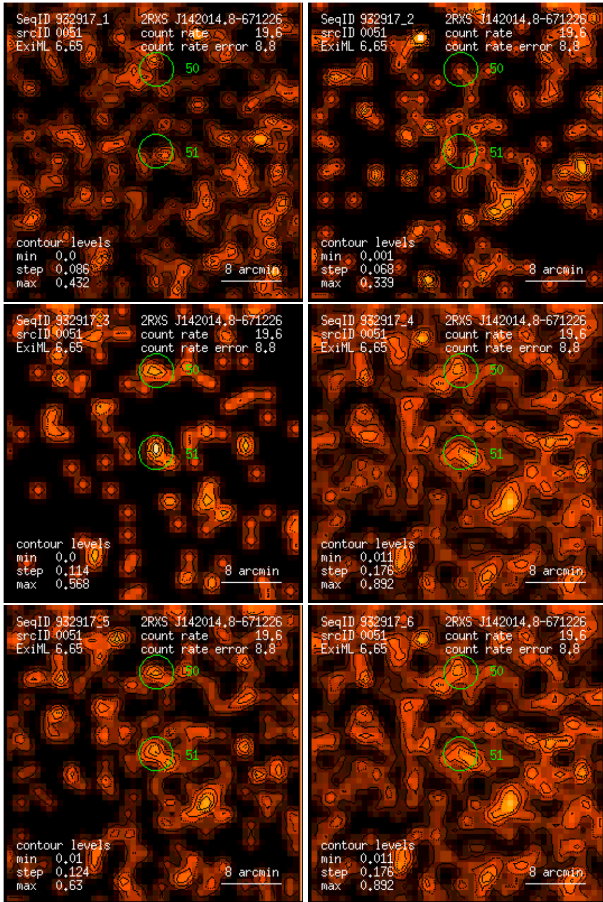
Figure 51: RASS 932917: detection 0051: band rate images, Gaussian filter: (1) PSPC channels 11 – 41, (2) 52 – 90, (3) 91 – 201, (4) 11 – 235, (5) 52 – 201, (6) 11 – 201. Broad band rates in counts/ks. Band rate contour levels in counts/ks/arcmin 2 .
