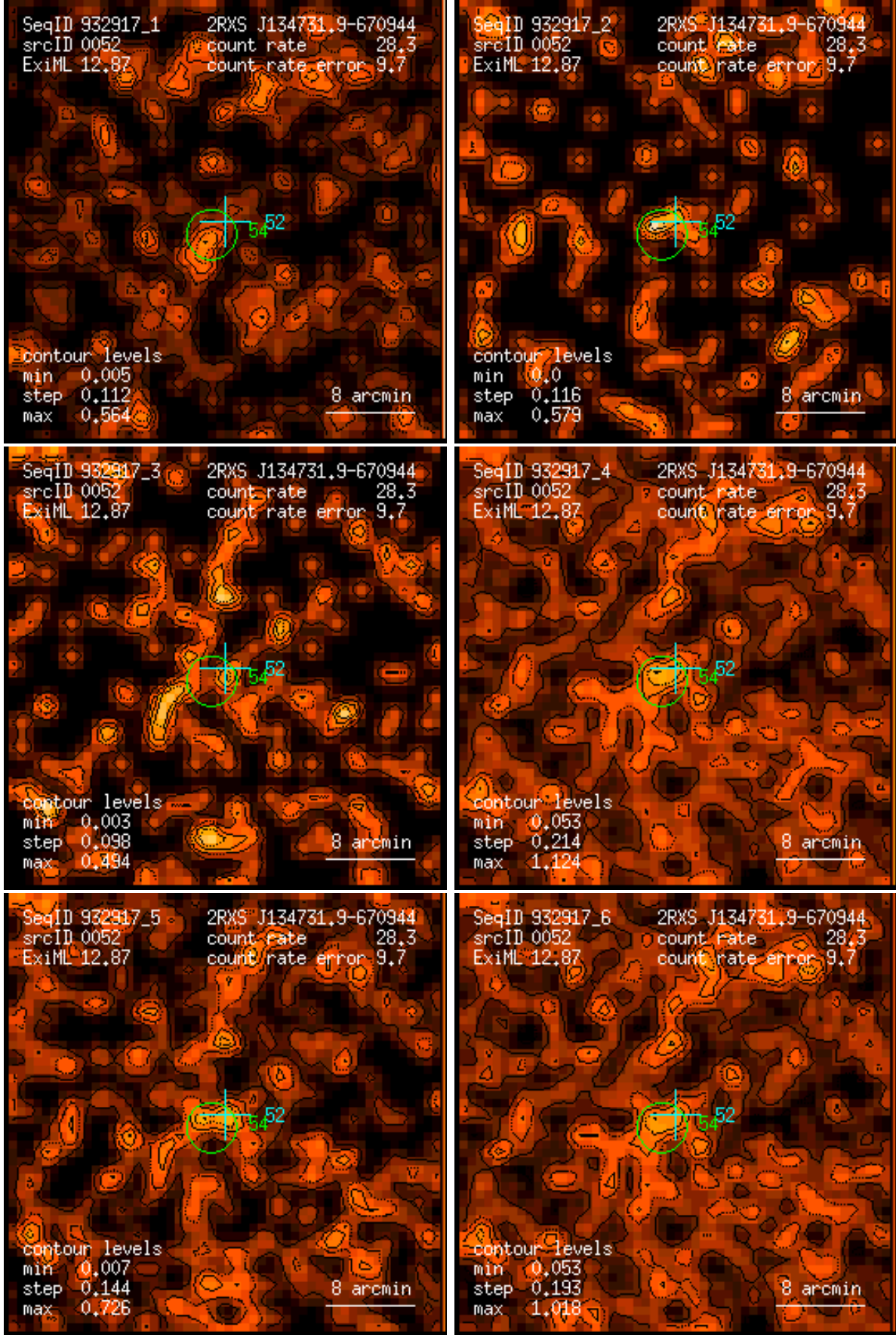
Figure 52: RASS 932917: detection 0052: band rate images, Gaussian filter: (1) PSPC channels 11 – 41, (2) 52 – 90, (3) 91 – 201, (4) 11 – 235, (5) 52 – 201, (6) 11 – 201. Broad band rates in counts/ks. Band rate contour levels in counts/ks/arcmin 2 .
