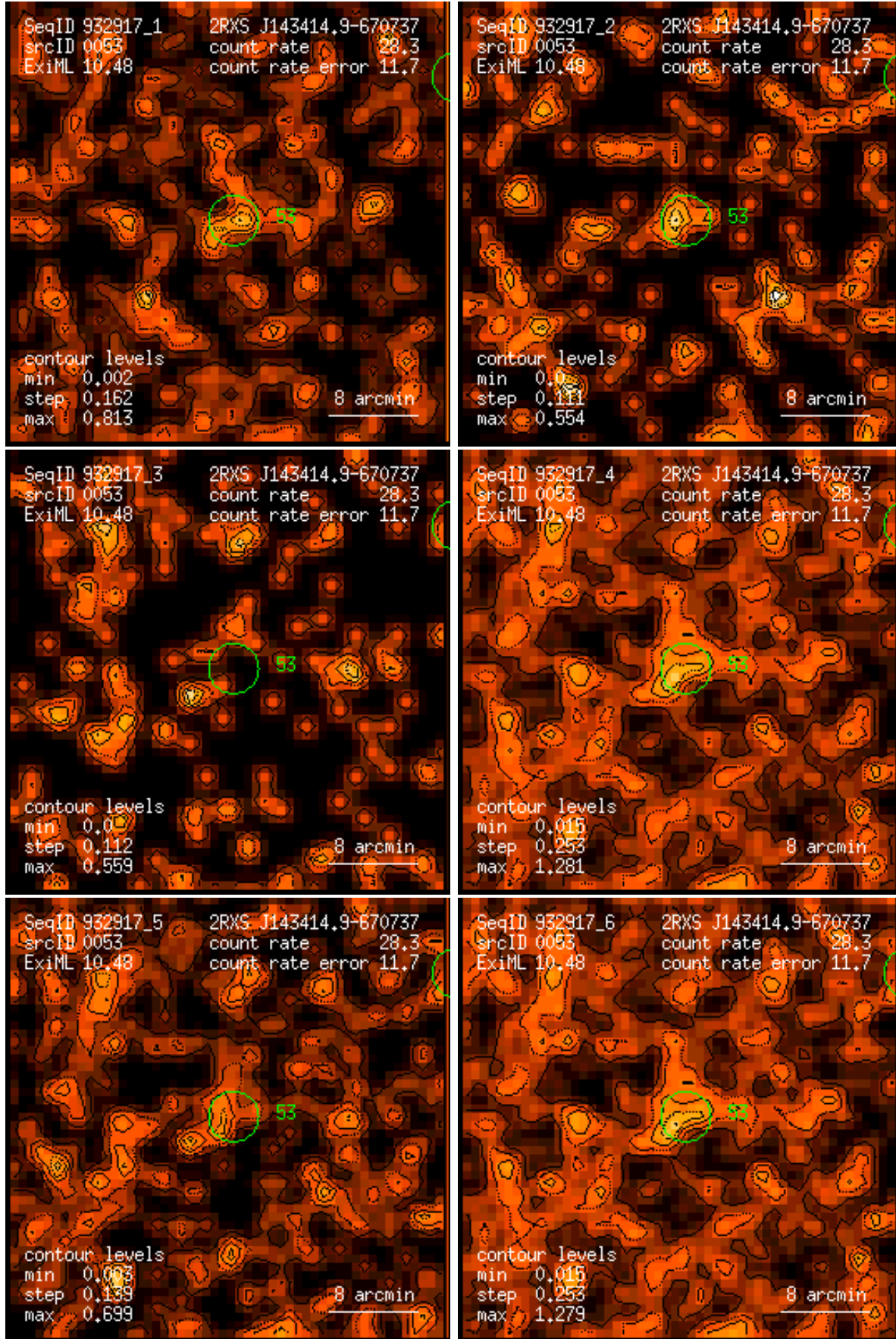
Figure 53: RASS 932917: detection 0053: band rate images, Gaussian filter: (1) PSPC channels 11 – 41, (2) 52 – 90, (3) 91 – 201, (4) 11 – 235, (5) 52 – 201, (6) 11 – 201. Broad band rates in counts/ks. Band rate contour levels in counts/ks/arcmin 2 .
