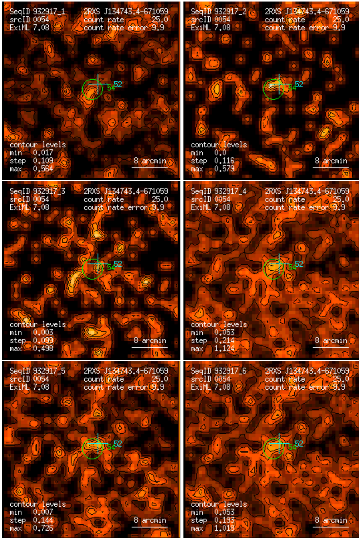
Figure 54: RASS 932917: detection 0054: band rate images, Gaussian filter: (1) PSPC channels 11 – 41, (2) 52 – 90, (3) 91 – 201, (4) 11 – 235, (5) 52 – 201, (6) 11 – 201. Broad band rates in counts/ks. Band rate contour levels in counts/ks/arcmin 2 .
