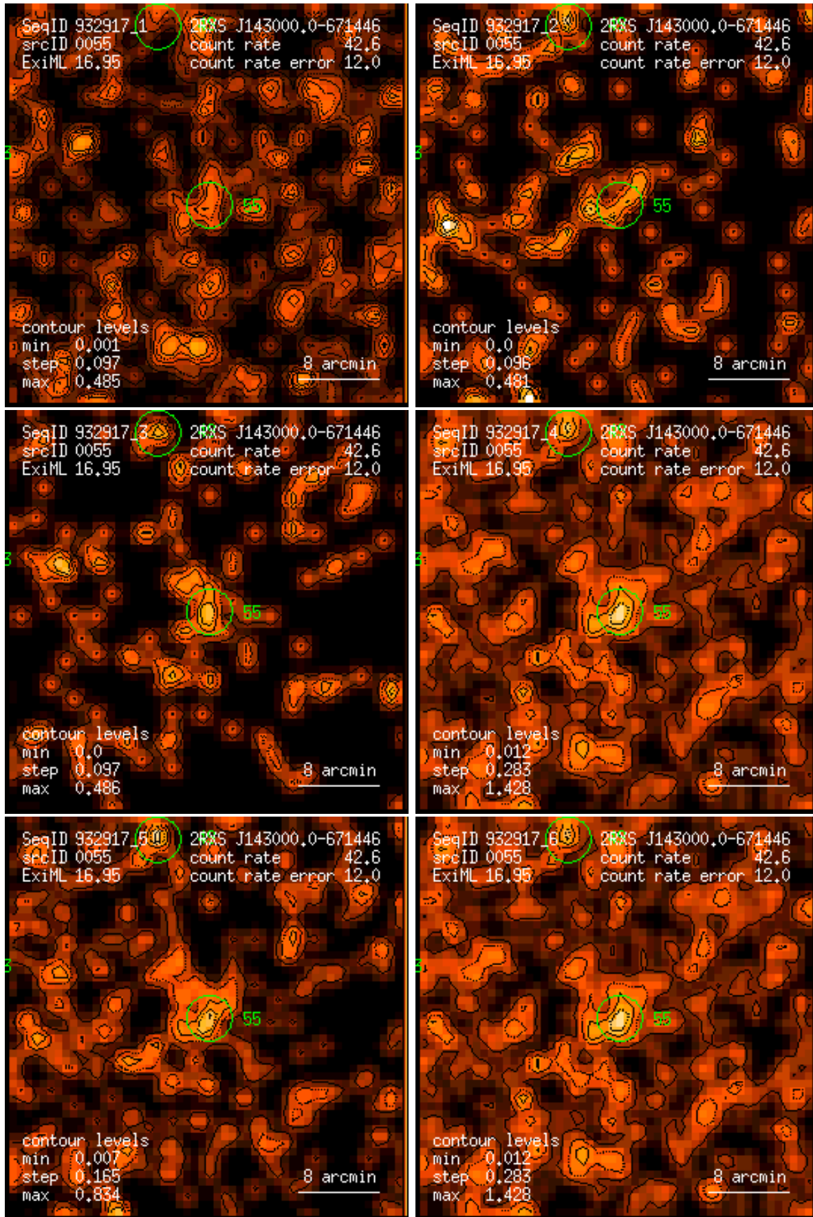
Figure 55: RASS 932917: detection 0055: band rate images, Gaussian filter: (1) PSPC channels 11 – 41, (2) 52 – 90, (3) 91 – 201, (4) 11 – 235, (5) 52 – 201, (6) 11 – 201. Broad band rates in counts/ks. Band rate contour levels in counts/ks/arcmin 2 .
