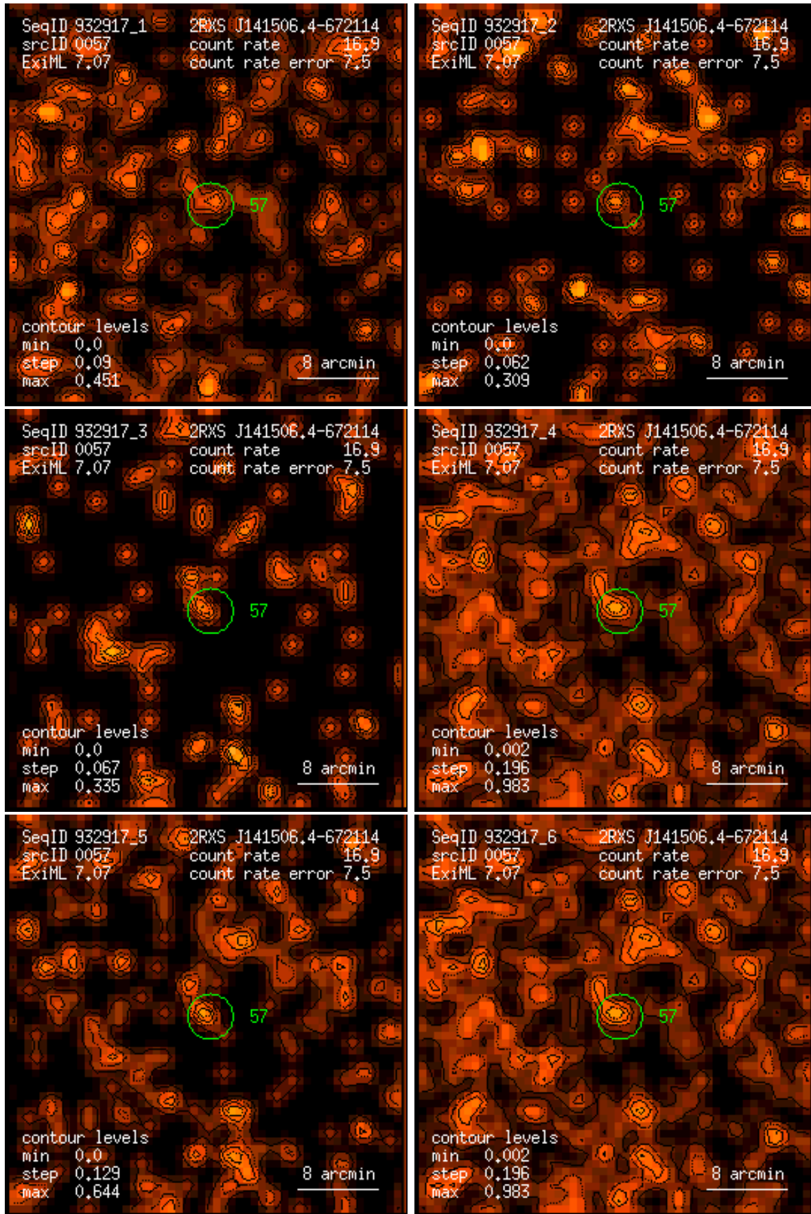
Figure 57: RASS 932917: detection 0057: band rate images, Gaussian filter: (1) PSPC channels 11 – 41, (2) 52 – 90, (3) 91 – 201, (4) 11 – 235, (5) 52 – 201, (6) 11 – 201. Broad band rates in counts/ks. Band rate contour levels in counts/ks/arcmin 2 .
