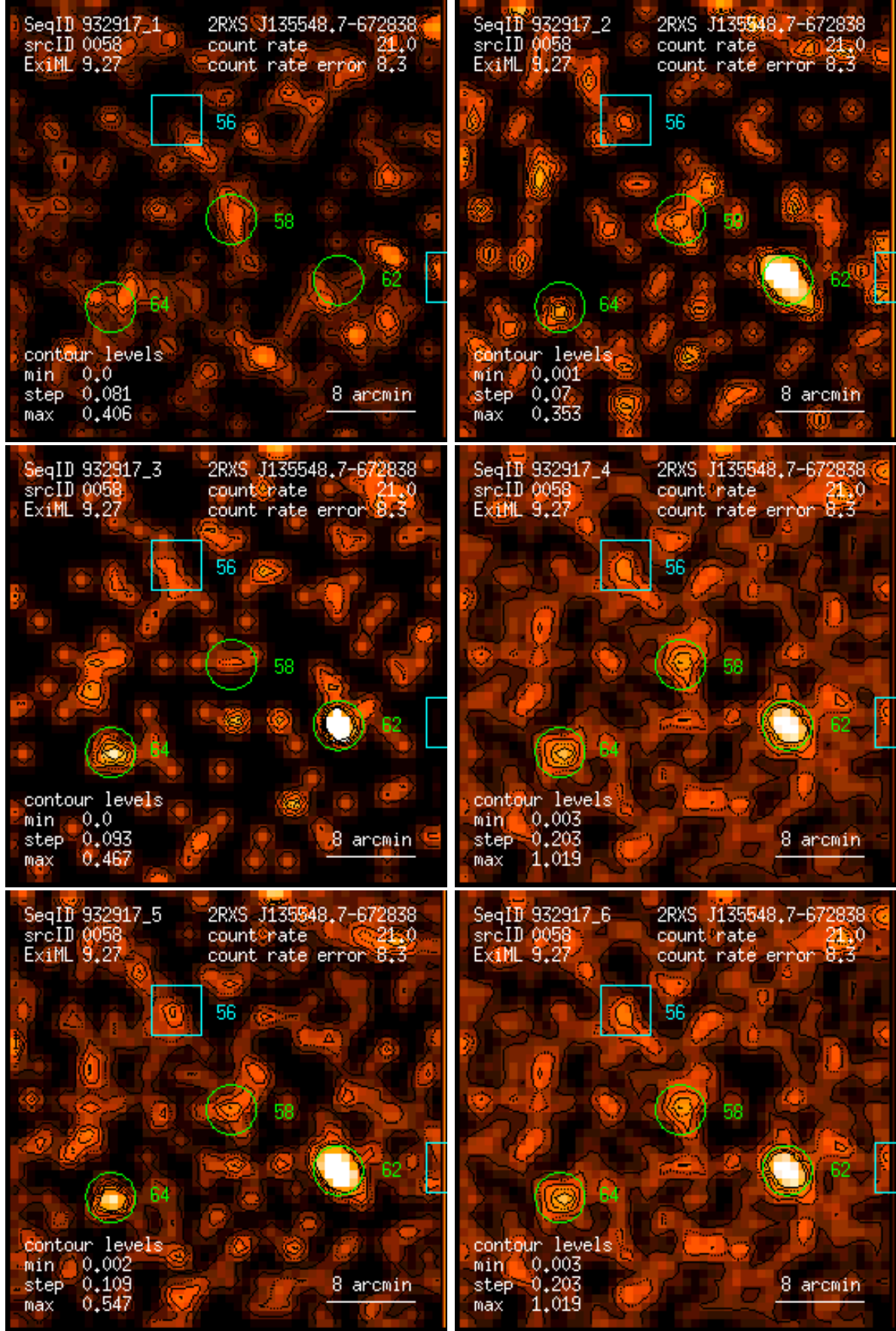
Figure 58: RASS 932917: detection 0058: band rate images, Gaussian filter: (1) PSPC channels 11 – 41, (2) 52 – 90, (3) 91 – 201, (4) 11 – 235, (5) 52 – 201, (6) 11 – 201. Broad band rates in counts/ks. Band rate contour levels in counts/ks/arcmin 2 .
