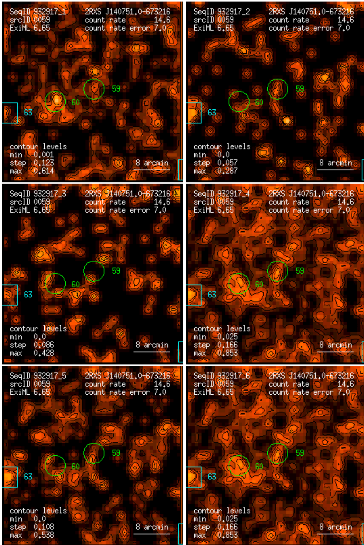
Figure 59: RASS 932917: detection 0059: band rate images, Gaussian filter: (1) PSPC channels 11 – 41, (2) 52 – 90, (3) 91 – 201, (4) 11 – 235, (5) 52 – 201, (6) 11 – 201. Broad band rates in counts/ks. Band rate contour levels in counts/ks/arcmin 2 .
