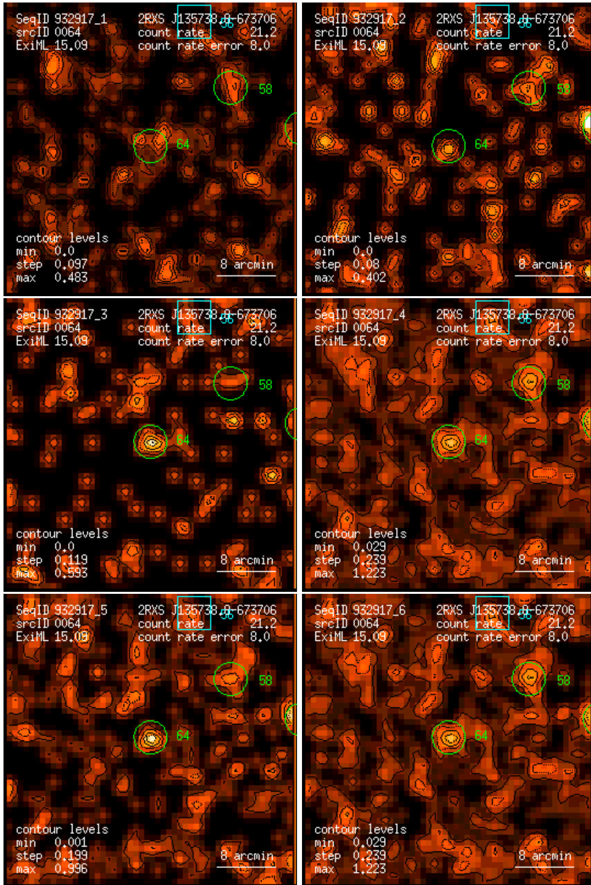
Figure 64: RASS 932917: detection 0064: band rate images, Gaussian filter: (1) PSPC channels 11 – 41, (2) 52 – 90, (3) 91 – 201, (4) 11 – 235, (5) 52 – 201, (6) 11 – 201. Broad band rates in counts/ks. Band rate contour levels in counts/ks/arcmin 2 .
