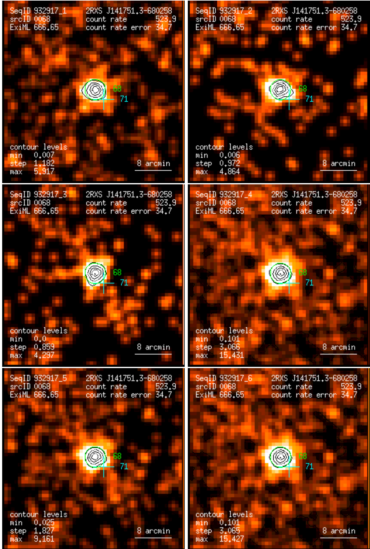
Figure 68: RASS 932917: detection 0068: band rate images, Gaussian filter: (1) PSPC channels 11 – 41, (2) 52 – 90, (3) 91 – 201, (4) 11 – 235, (5) 52 – 201, (6) 11 – 201. Broad band rates in counts/ks. Band rate contour levels in counts/ks/arcmin 2 .
