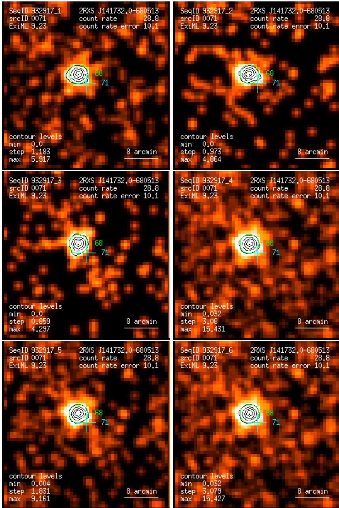
Figure 71: RASS 932917: detection 0071: band rate images, Gaussian filter: (1) PSPC channels 11 – 41, (2) 52 – 90, (3) 91 – 201, (4) 11 – 235, (5) 52 – 201, (6) 11 – 201. Broad band rates in counts/ks. Band rate contour levels in counts/ks/arcmin 2 .
