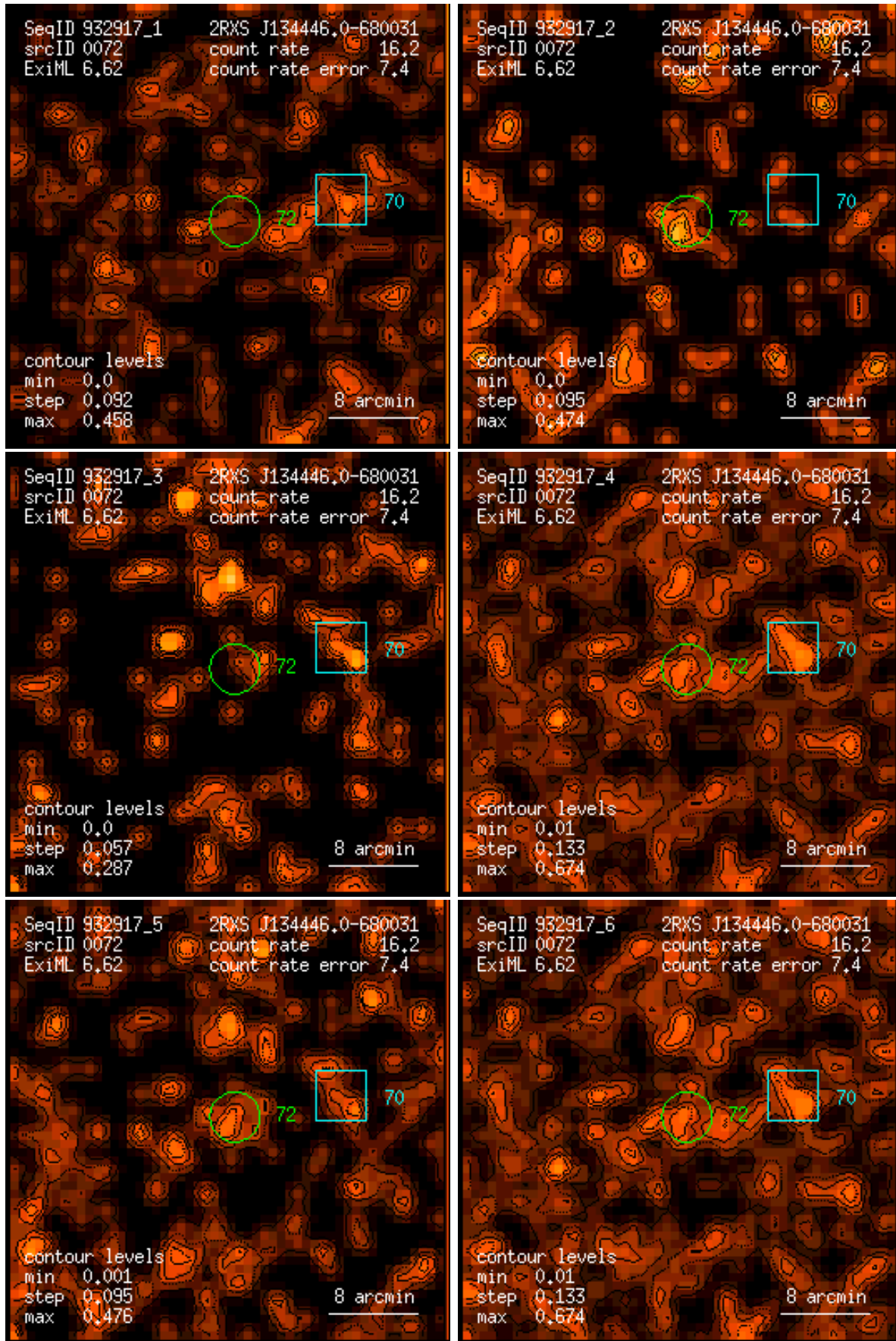
Figure 72: RASS 932917: detection 0072: band rate images, Gaussian filter: (1) PSPC channels 11 – 41, (2) 52 – 90, (3) 91 – 201, (4) 11 – 235, (5) 52 – 201, (6) 11 – 201. Broad band rates in counts/ks. Band rate contour levels in counts/ks/arcmin 2 .
